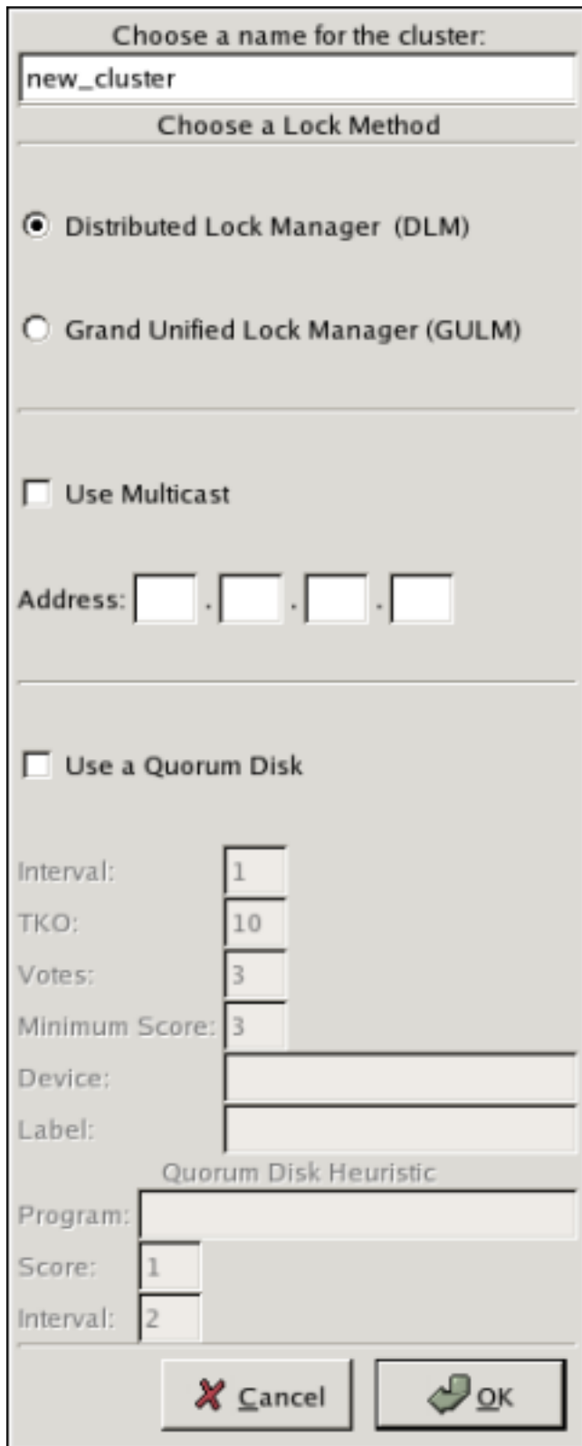
Figure 5.2. Creating A New Configuration
