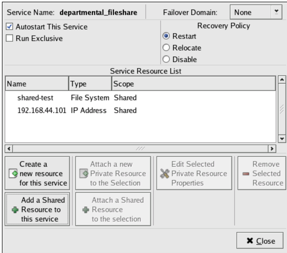
Figure 5.12. Adding a Cluster Service
