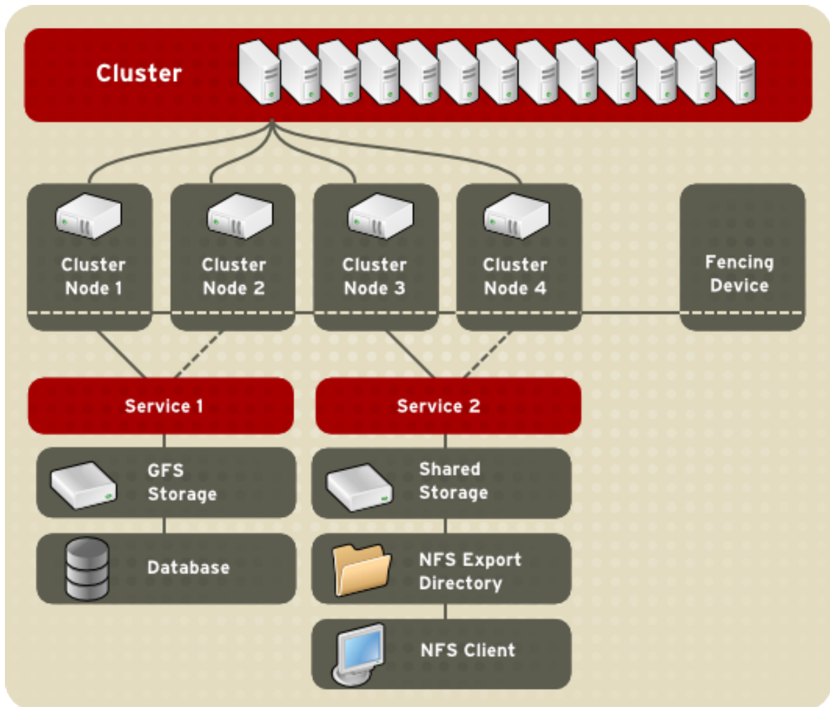
Figure 1.2. Cluster Configuration Structure
