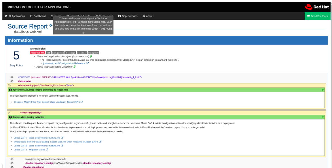
Figure 2.2. Rule match
