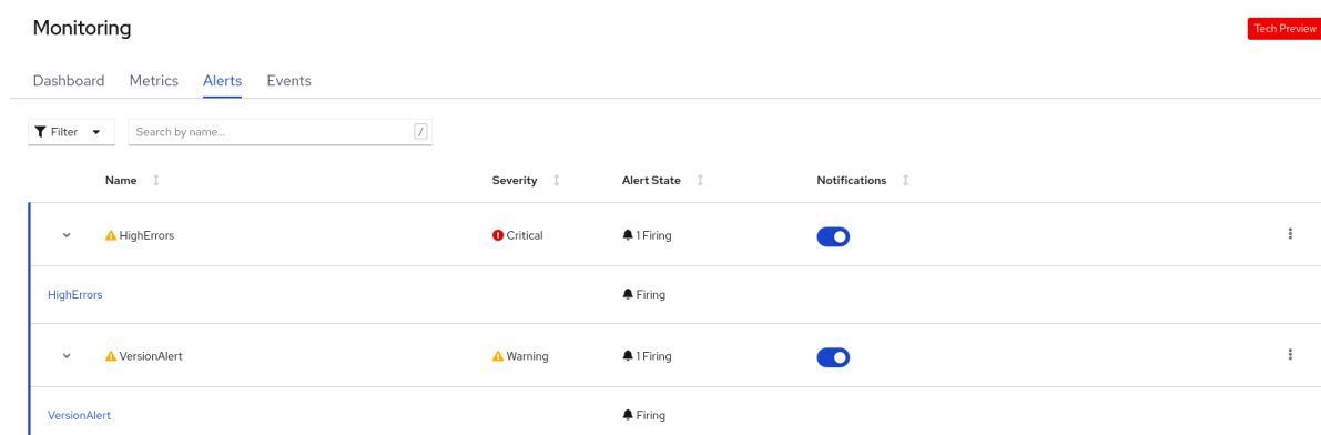
Figure 11.3. Monitoring alerts
