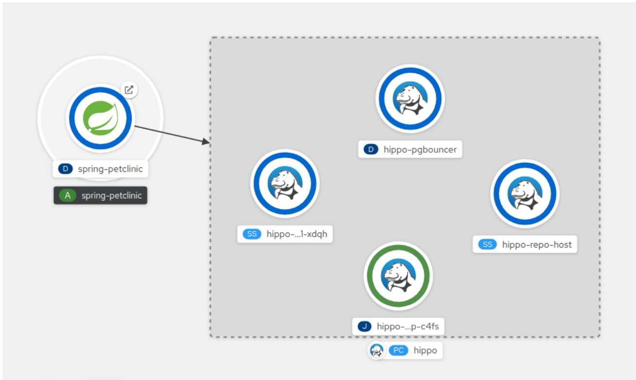
Figure 6.5. Binding connector
