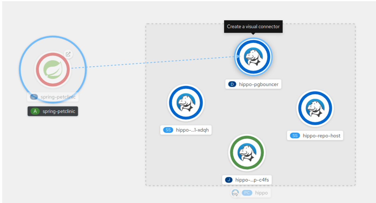
Figure 6.2. Visual connector
