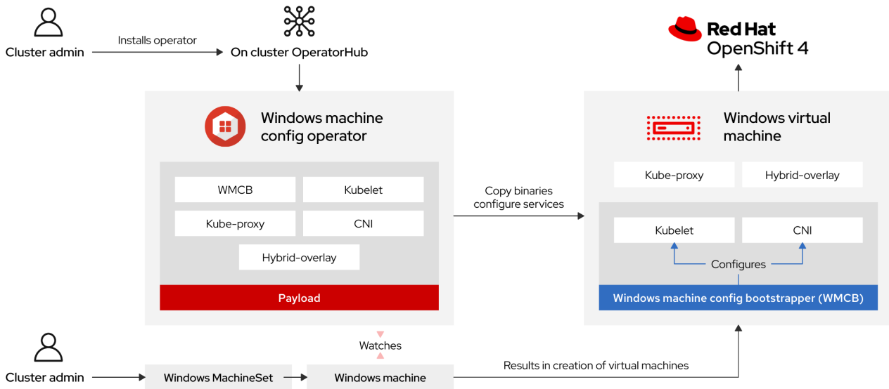
Figure 3.1. WMCO design
