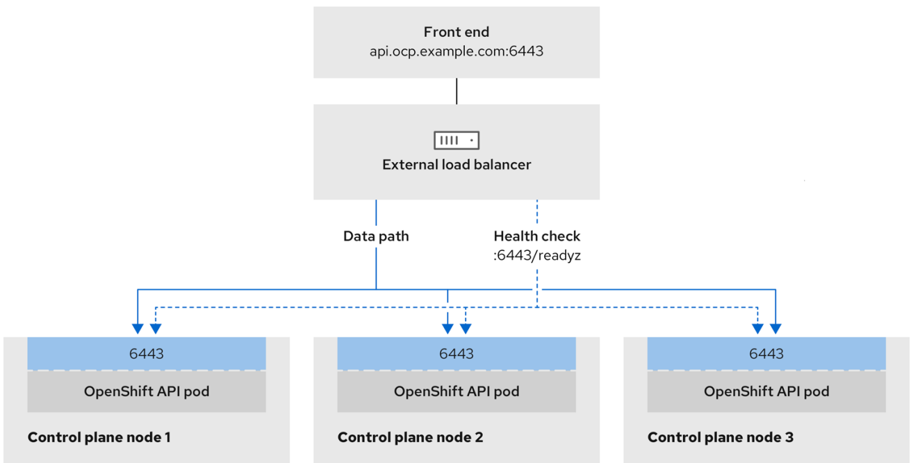
Figure 24.5. Example network workflow that shows an OpenShift API operating in an OpenShift Container Platform environment
