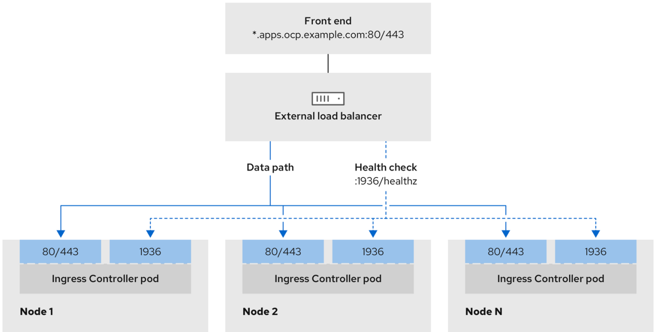
Figure 24.7. Example network workflow that shows an Ingress Controller operating in an OpenShift Container Platform environment
