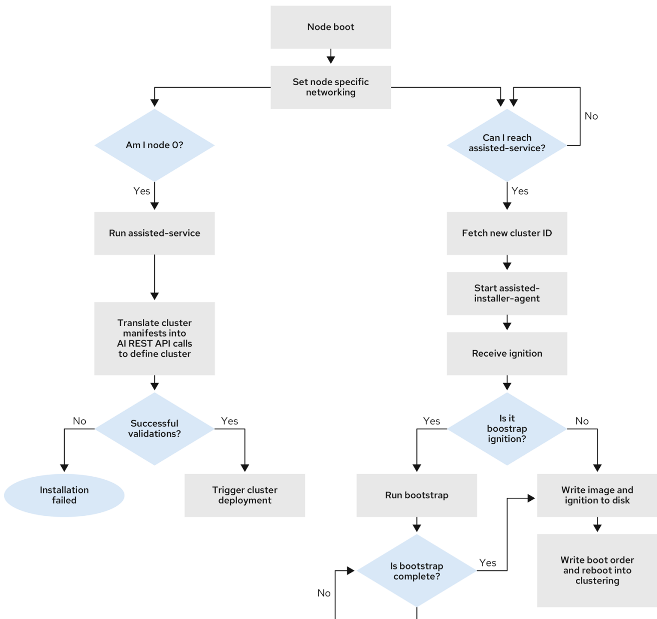
Figure 12.1. Node installation workflow
