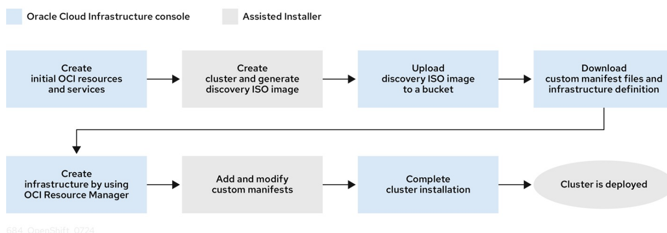
Figure 20.1. Workflow for using the Assisted Installer in a connected environment to install a cluster on OCI
