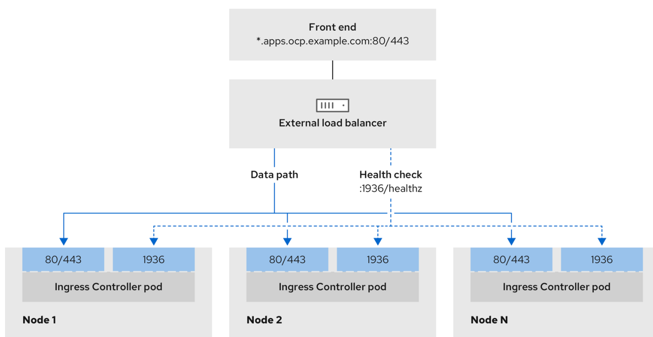
Figure 21.4. Example network workflow that shows an Ingress Controller operating in an OpenShift Container Platform environment
