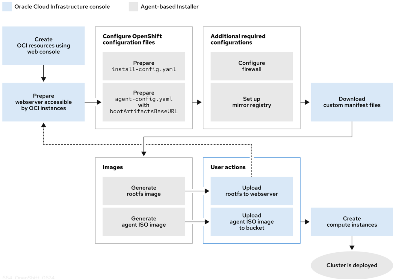
Figure 20.4. Workflow for using the Agent-based installer in a disconnected environment to install a cluster on OCI
