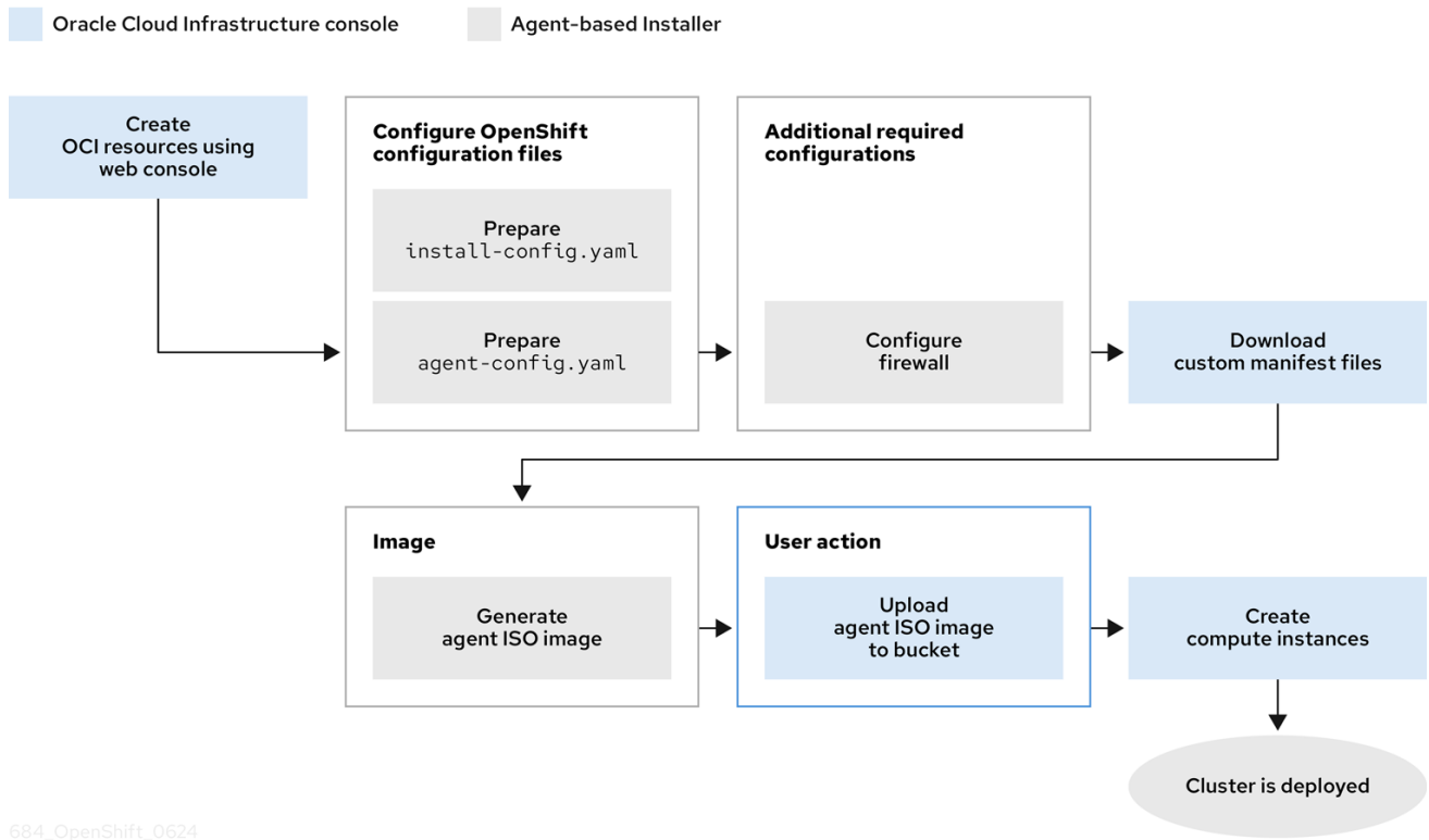
Figure 20.3. Workflow for using the Agent-based installer in a connected environment to install a cluster on OCI
