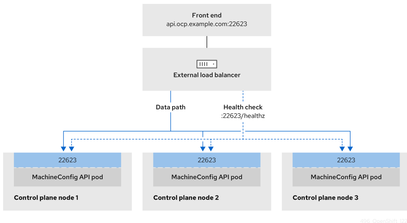
Figure 14.3. Example network workflow that shows an OpenShift MachineConfig API operating in an OpenShift Container Platform environment
