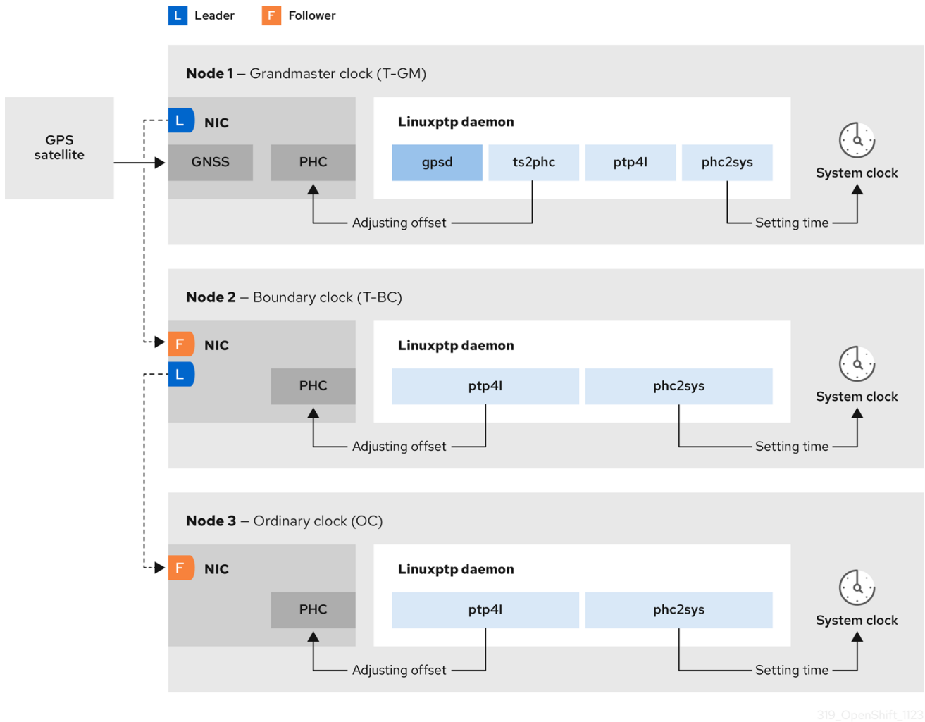
Figure 19.1. PTP nodes in the network
