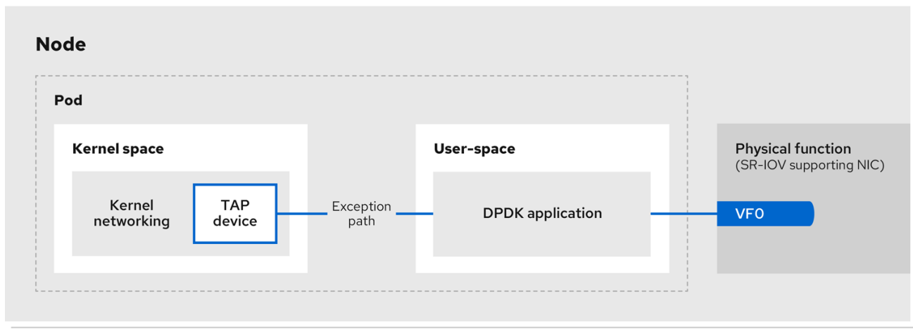
Figure 25.1. DPDK and TAP example configuration
