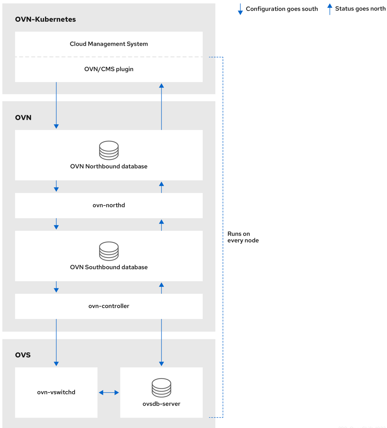
Figure 26.1. OVK-Kubernetes architecture
