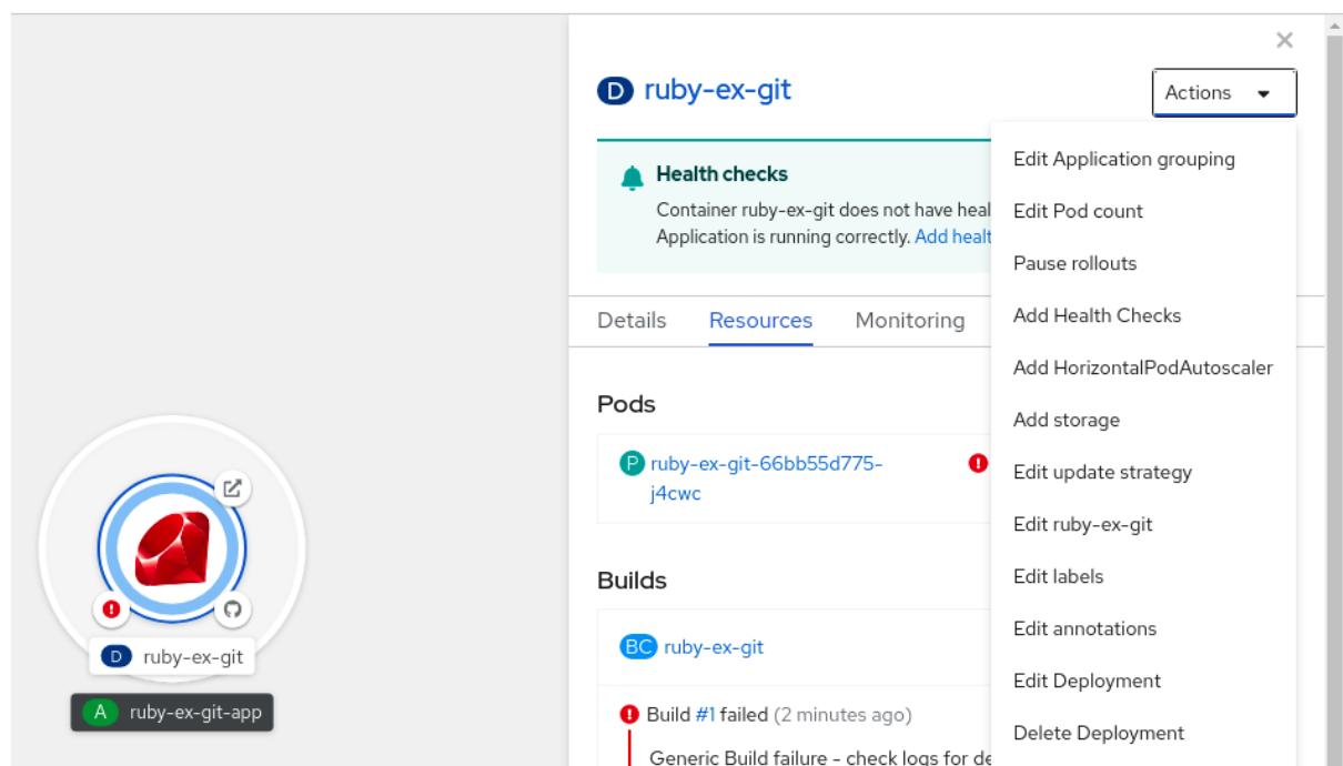
Figure 2.2. Add HorizontalPodAutoscaler
