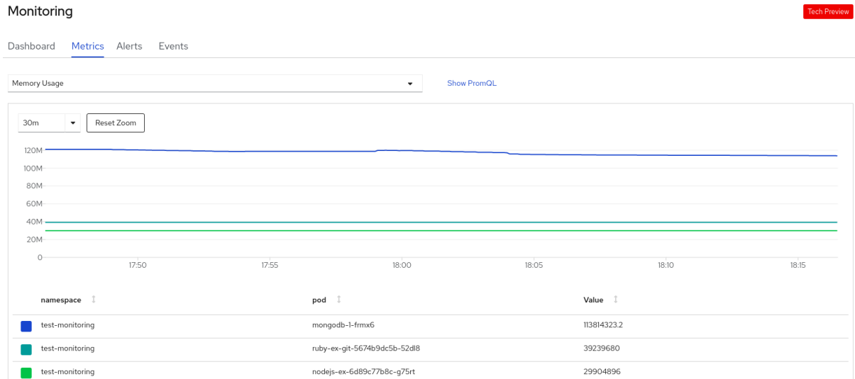
Figure 9.1. Monitoring metrics
