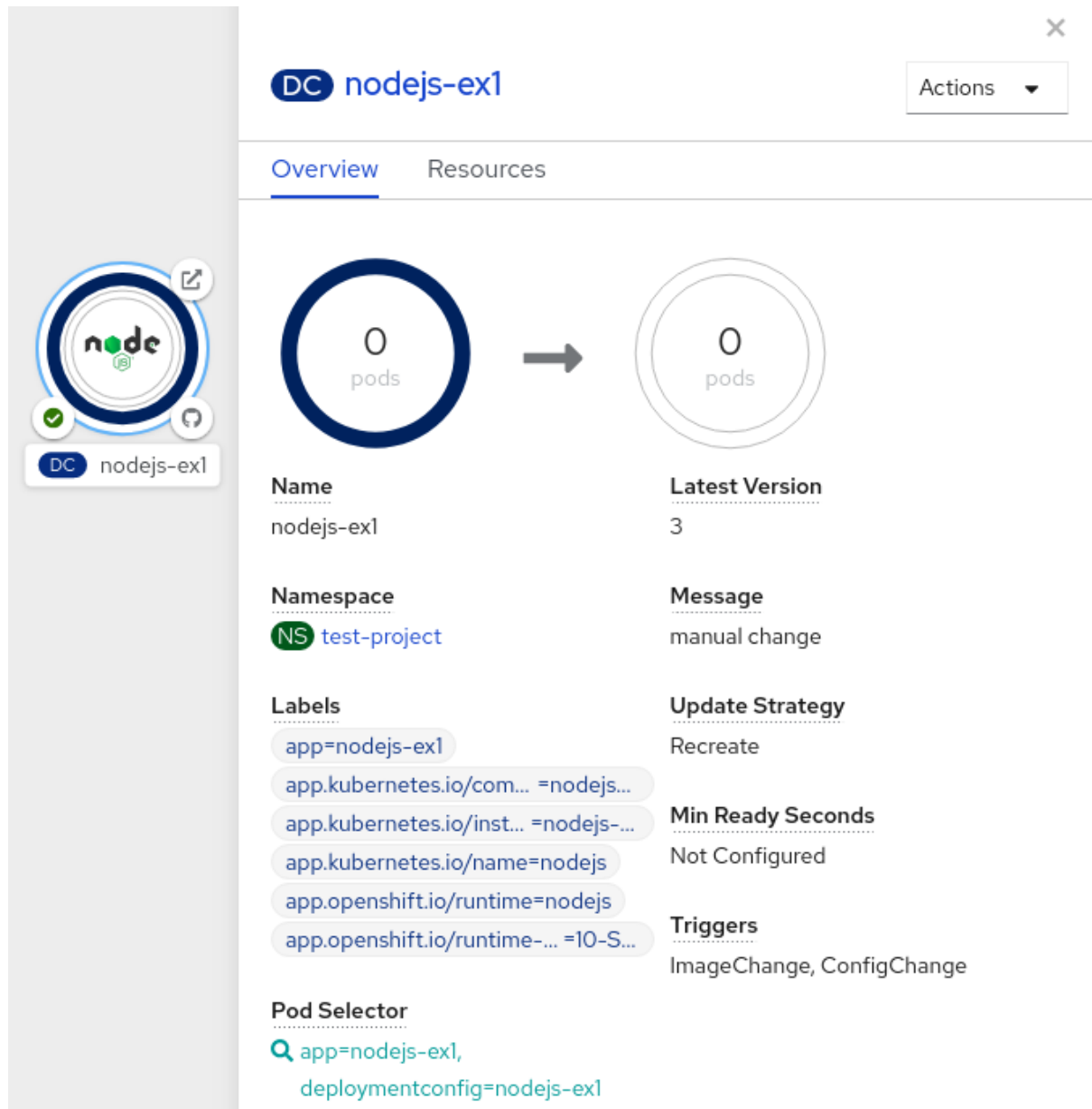
Figure 6.2. Recreate update
