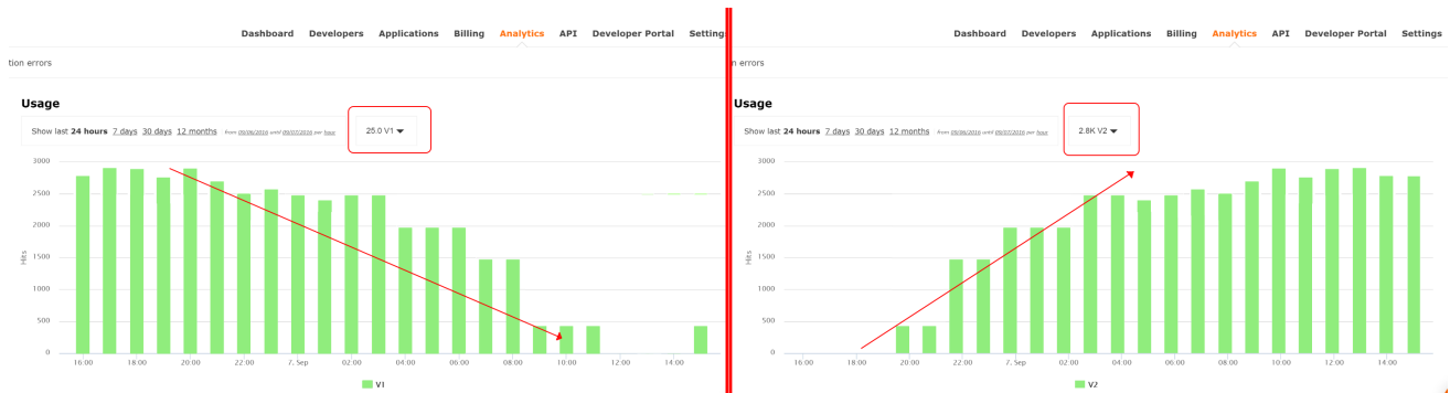
Figure 11.3. Versioning
