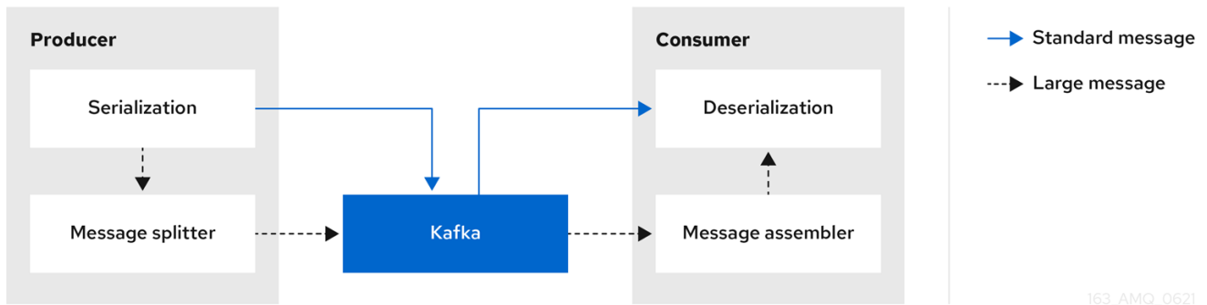
Figure 6.5. Inline messaging flow
