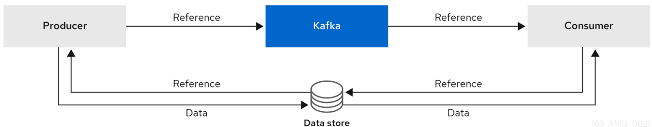
Figure 6.4. Reference-based messaging flow
