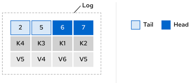
Figure 6.2. Log after compaction
