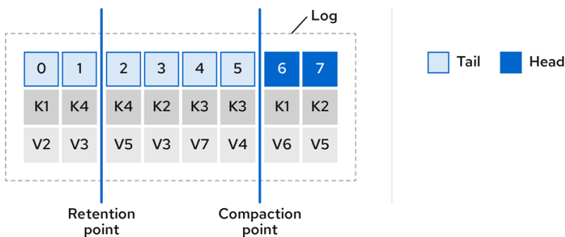
Figure 6.3. Log retention point and compaction point
