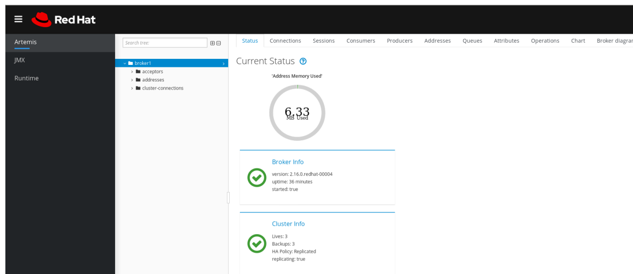
Figure 4.2. Status tab
