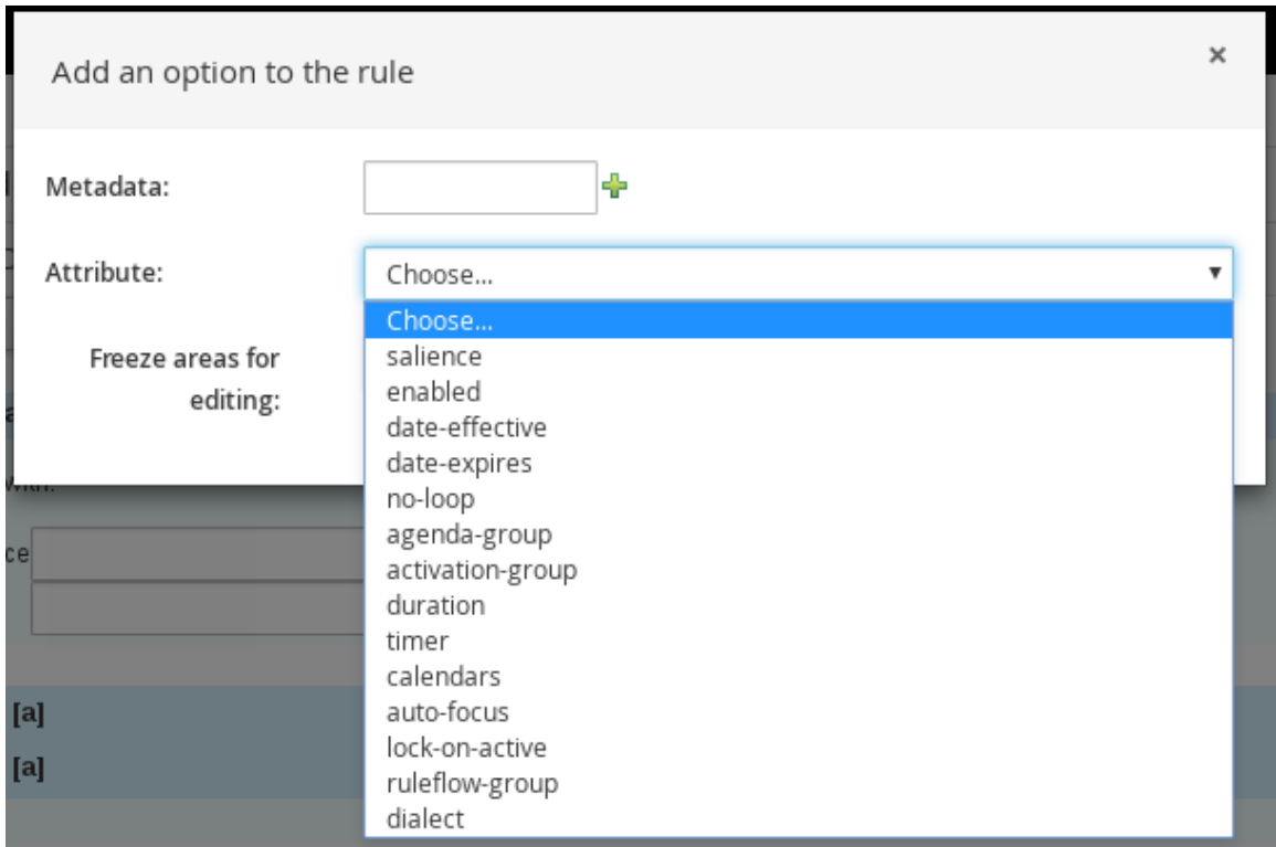
Figure 4.7. Rule options
