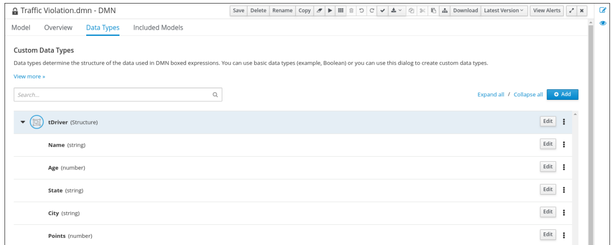
Figure 3.4. The tDriver custom data type
