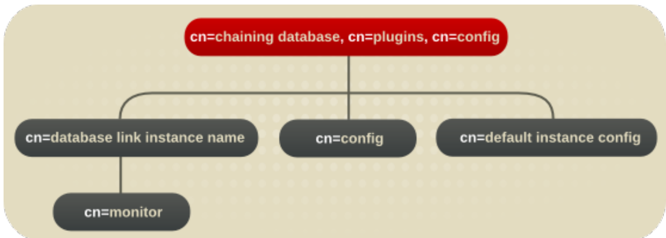
Figure 4.4. Database Link Plug-in
