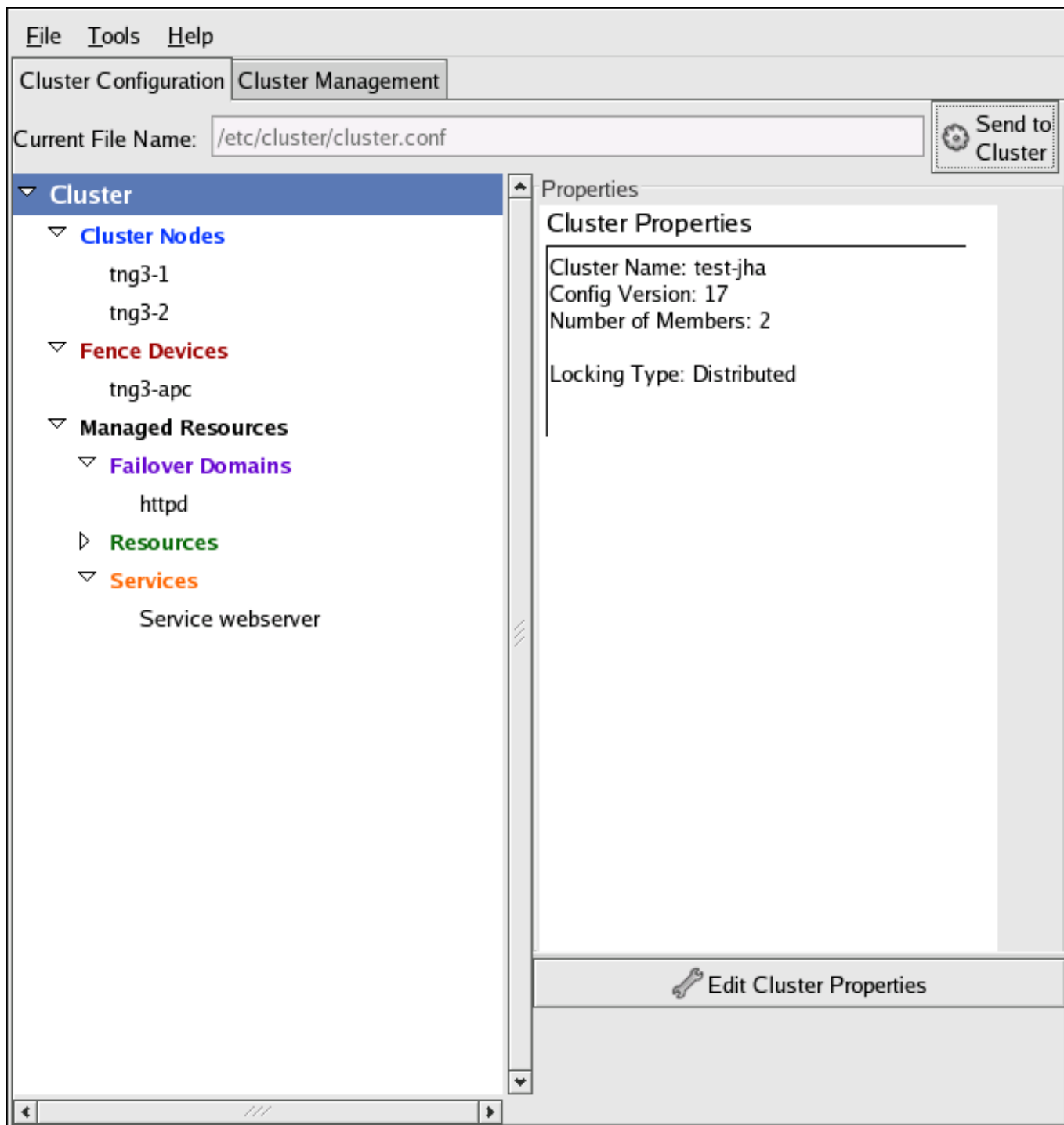
Figure 1.6. Cluster Configuration Tool
