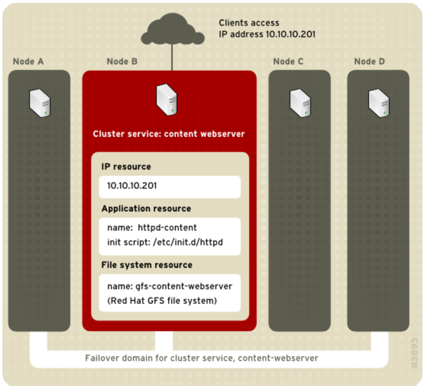
Figure 2.1. Web Server Cluster Service Example
