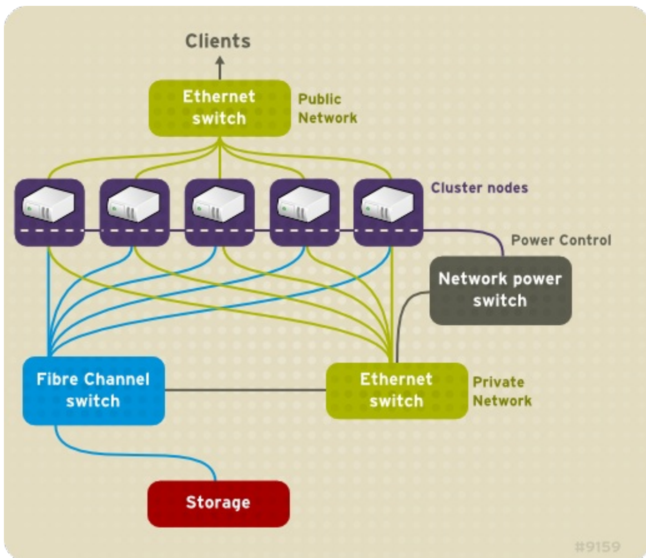
Figure 1.1. Red Hat Cluster Hardware Overview
