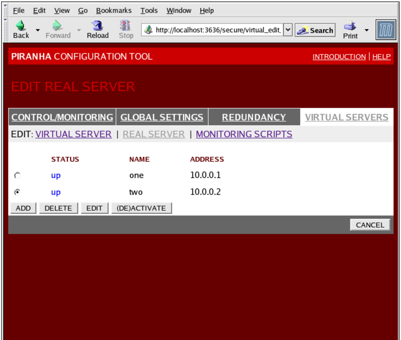
Figure 1.32. The REAL SERVER Subsection
