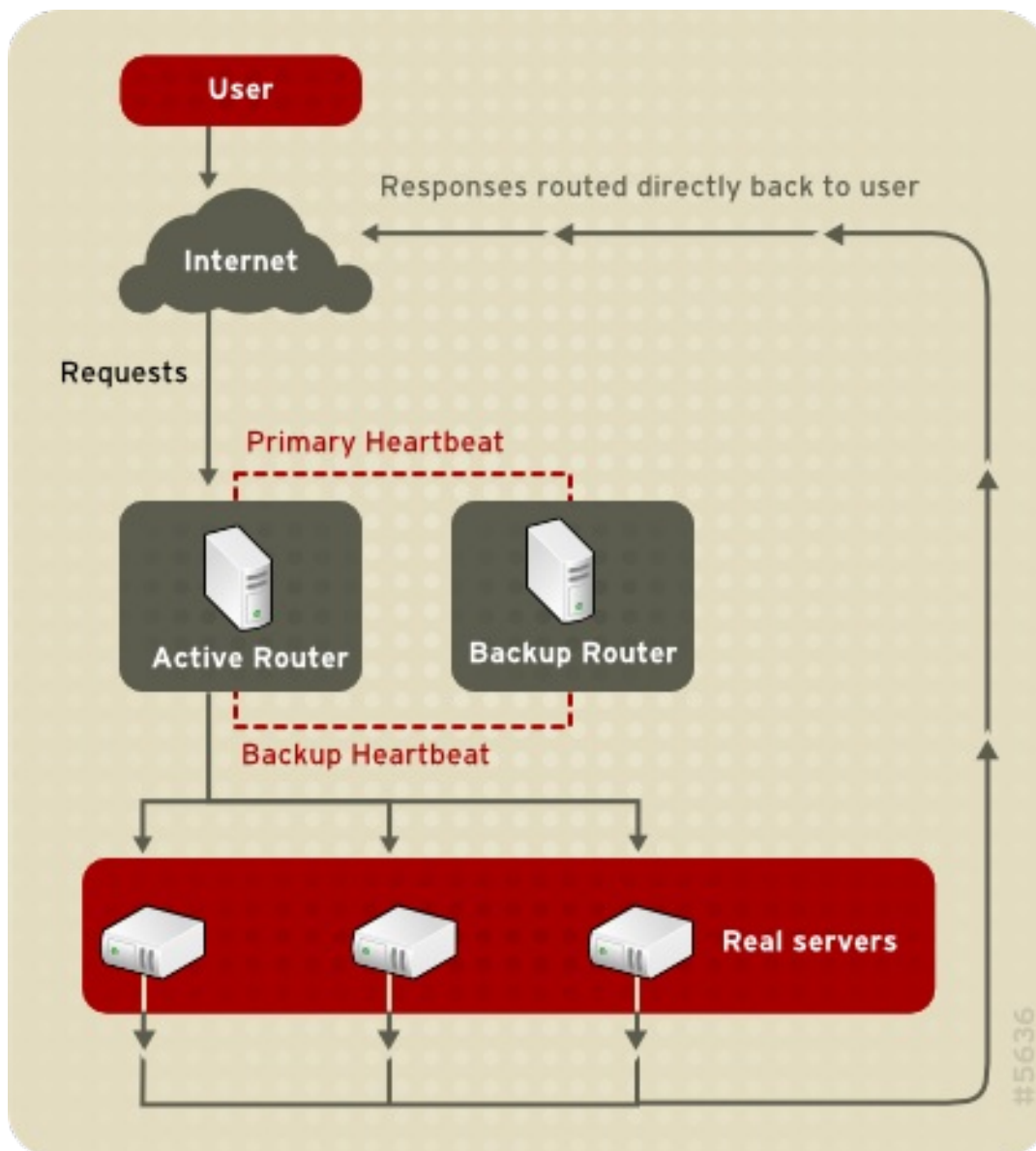
Figure 1.20. LVS Implemented with Direct Routing
