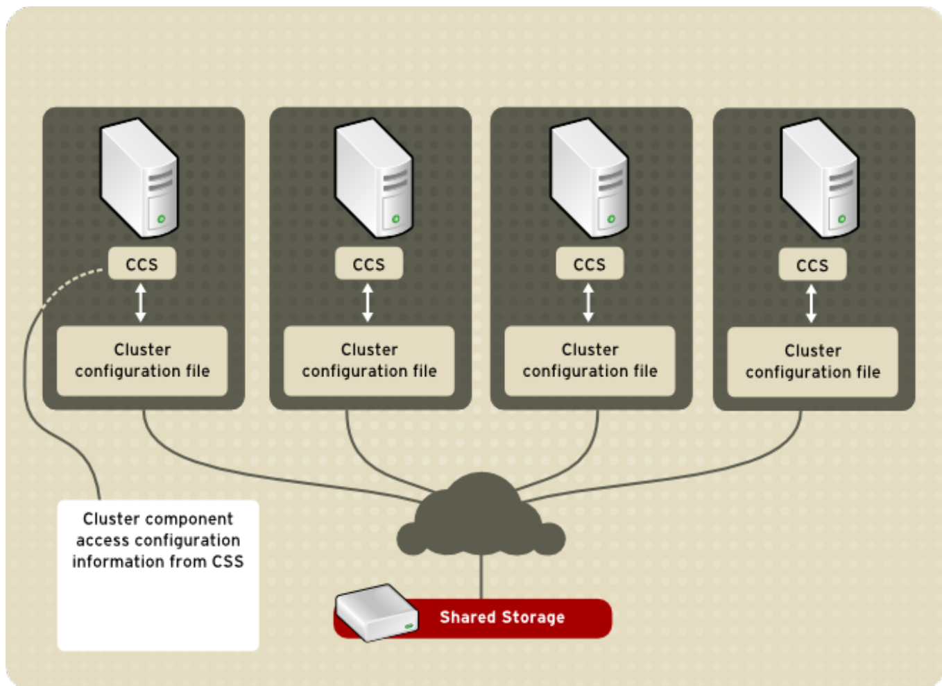
Figure 1.8. Accessing Configuration Information
