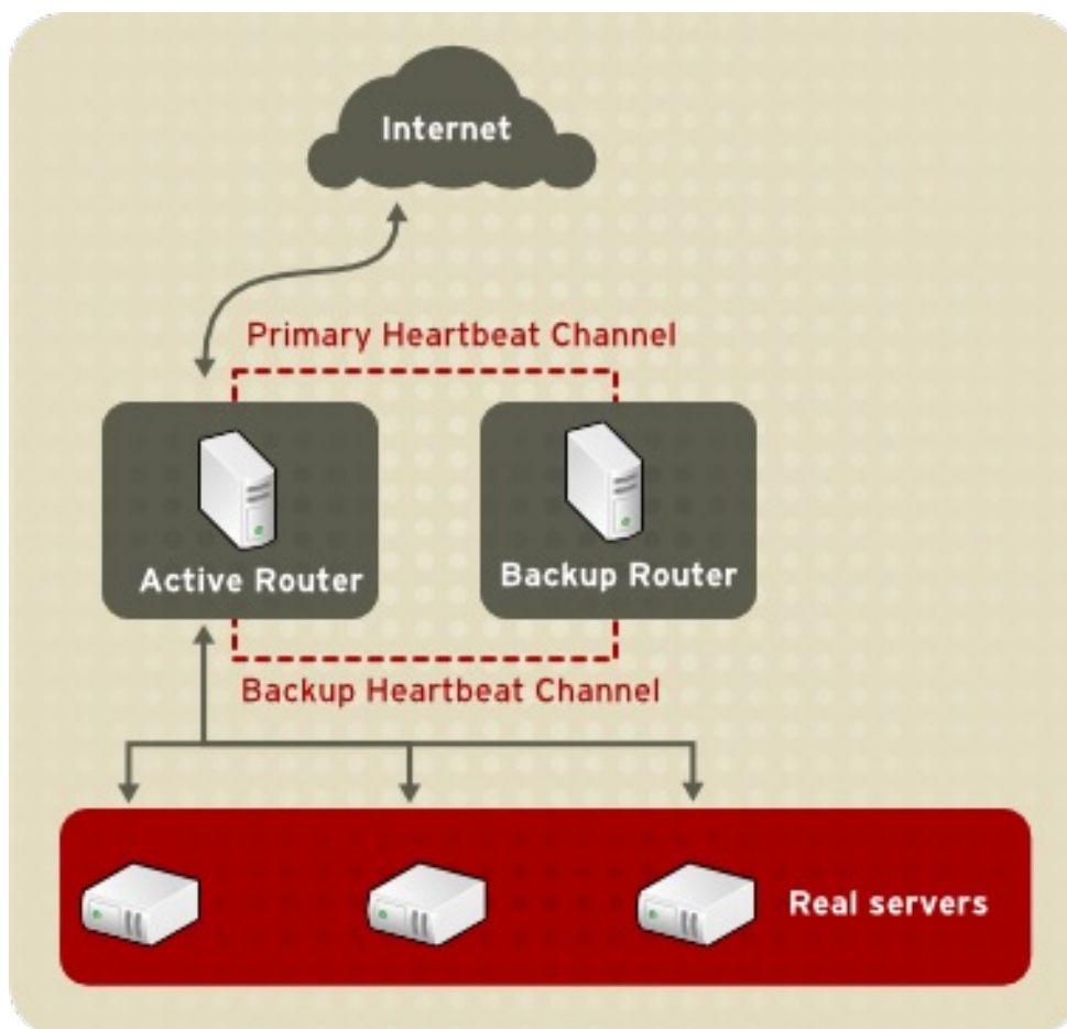
Figure 1.17. Two-Tier LVS Topology
