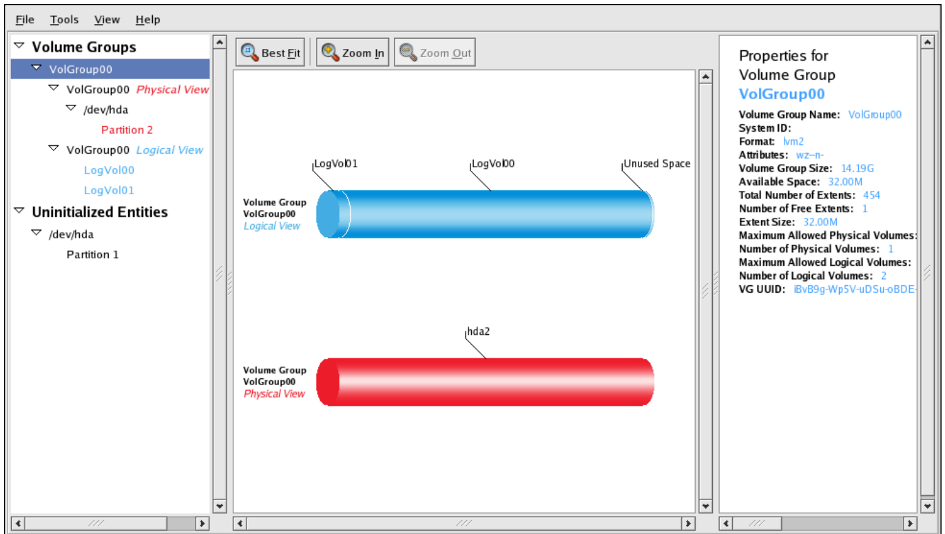
Figure 1.12. LVM Graphical User Interface
