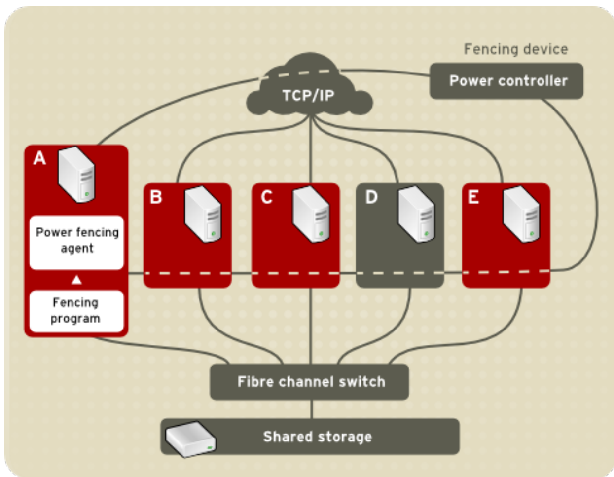
Figure 1.3. Power Fencing Example
