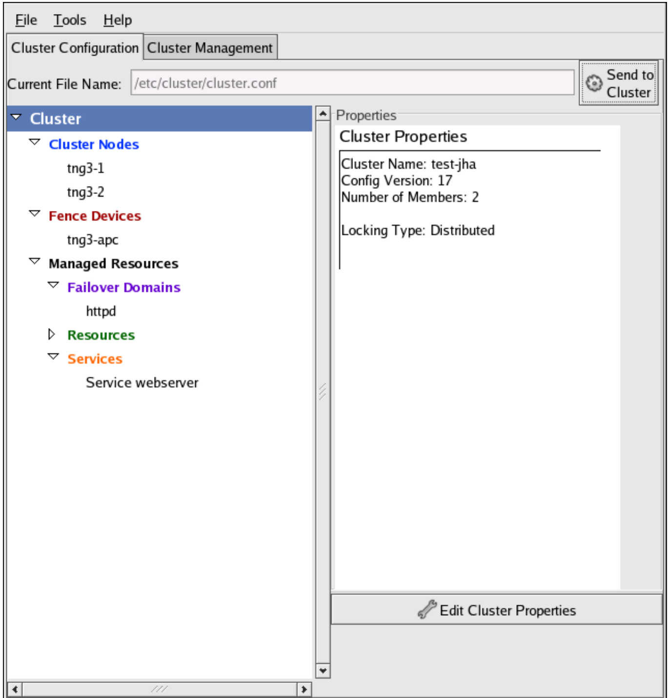
Figure 1.24. Cluster Configuration Tool
