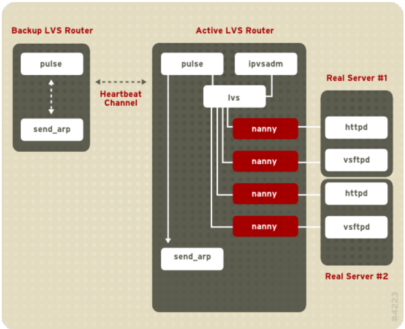
Figure 1.16. Components of a Running LVS Cluster
