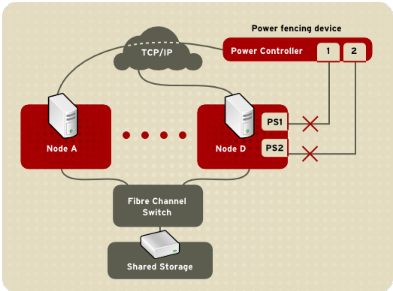
Figure 1.5. Fencing a Node with Dual Power Supplies
