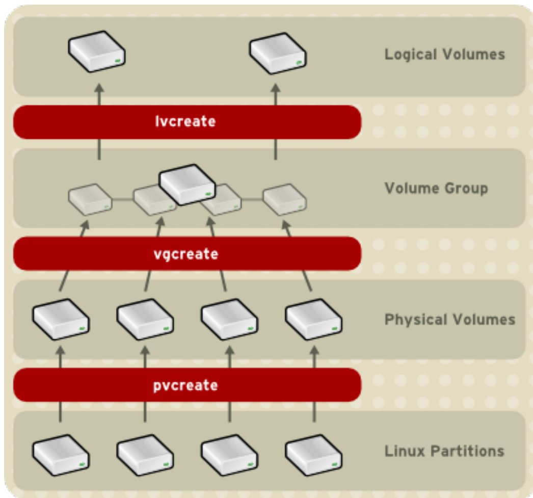
Figure 1.14. Creating Logical Volumes
