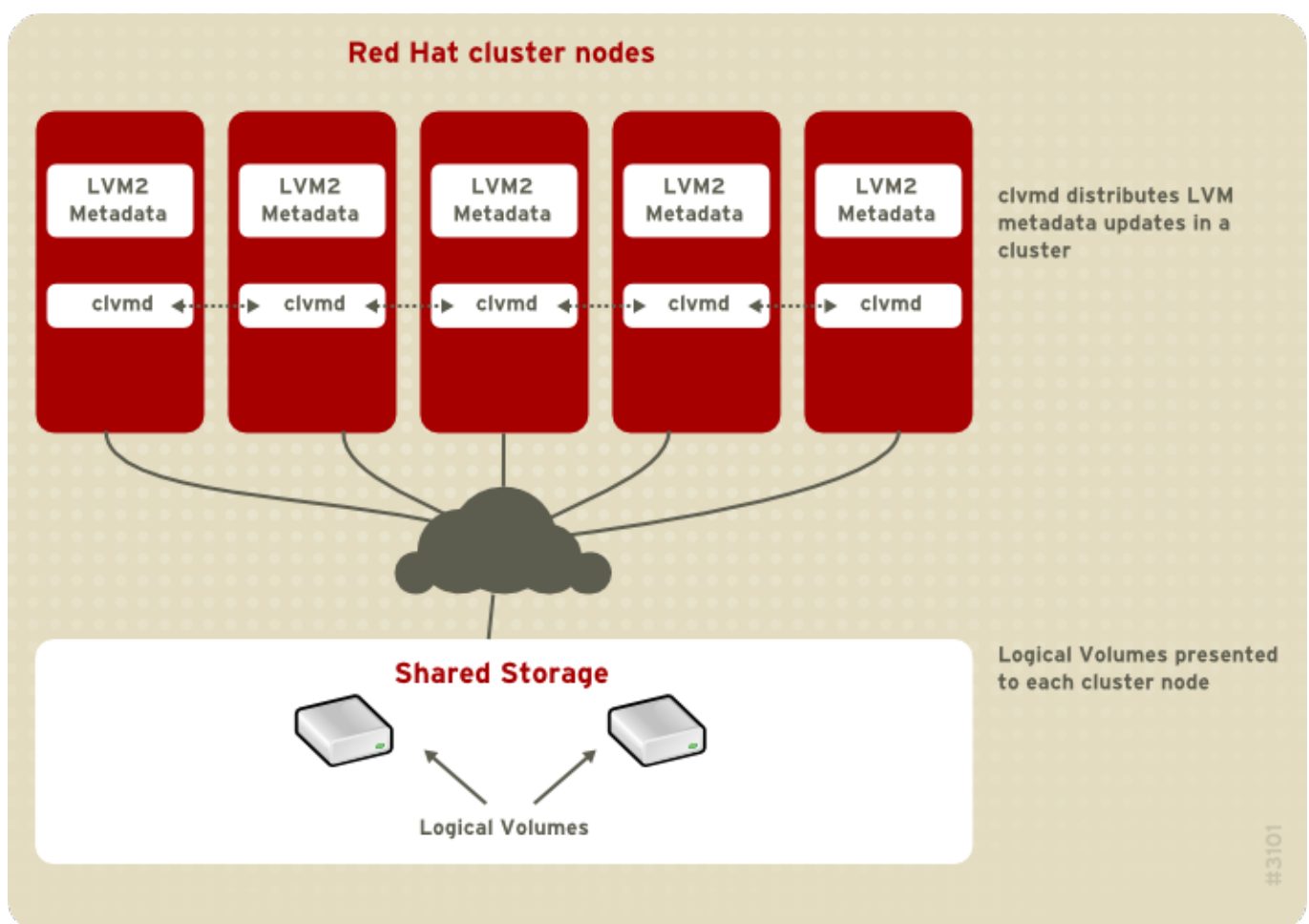
Figure 1.11. CLVM Overview
