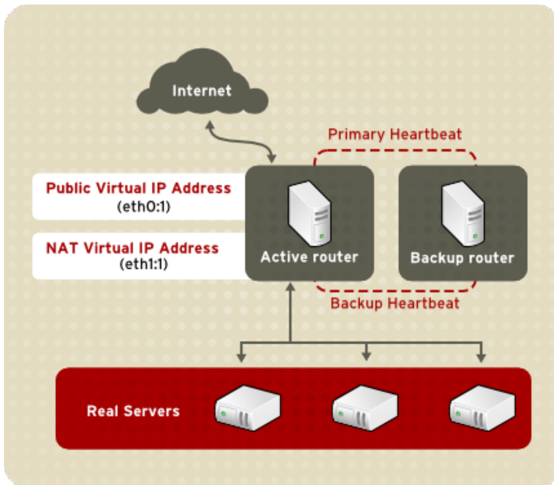
Figure 1.19. LVS Implemented with NAT Routing
