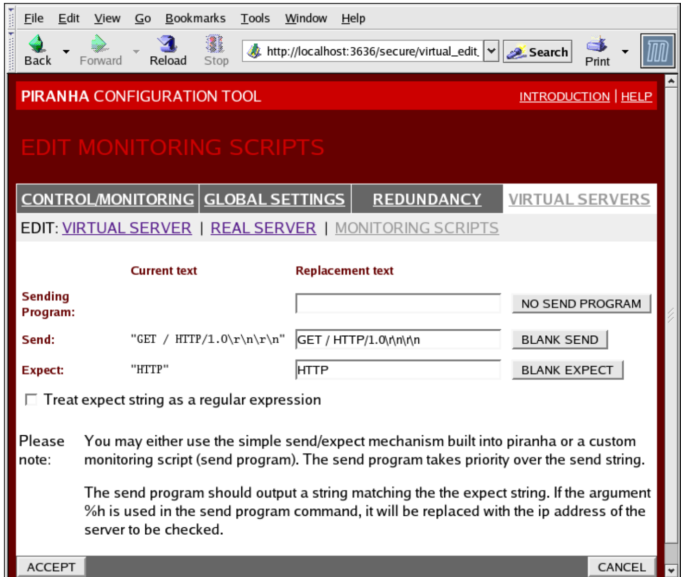
Figure 1.34. The EDIT MONITORING SCRIPTS Subsection
