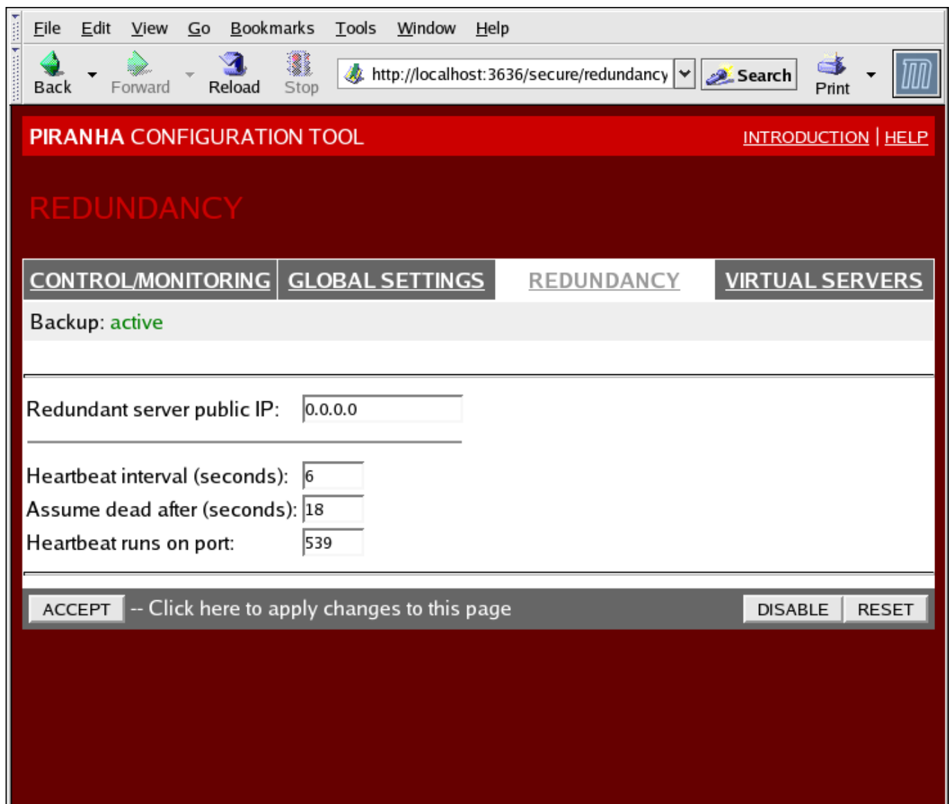
Figure 1.29. The REDUNDANCY Panel
