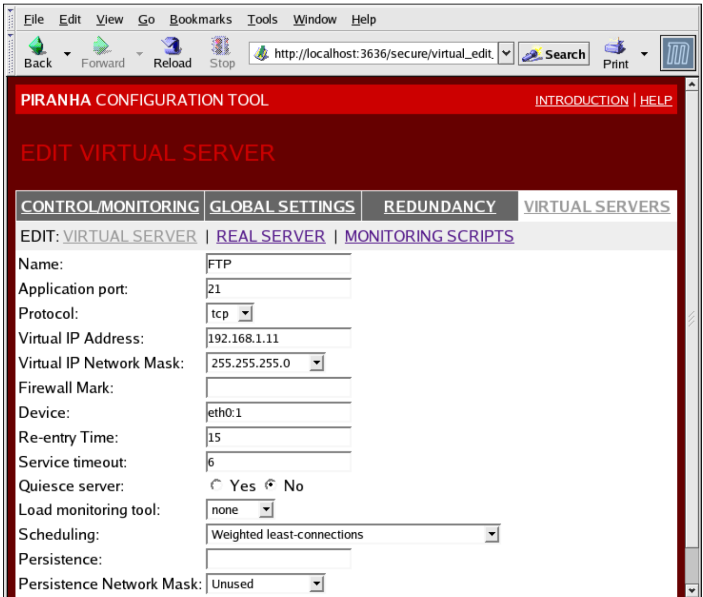
Figure 1.31. The VIRTUAL SERVERS Subsection
