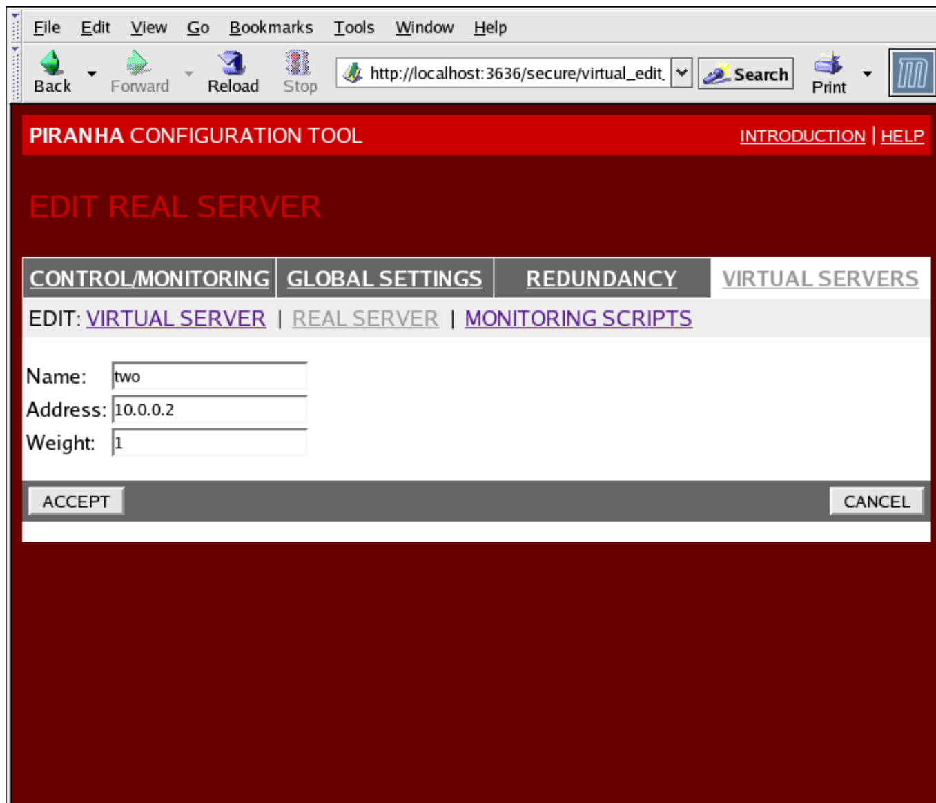
Figure 4.8. The REAL SERVER Configuration Panel
