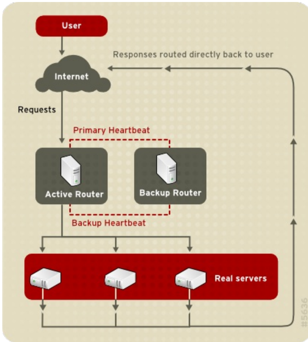
Figure 1.4. LVS Implemented with Direct Routing
