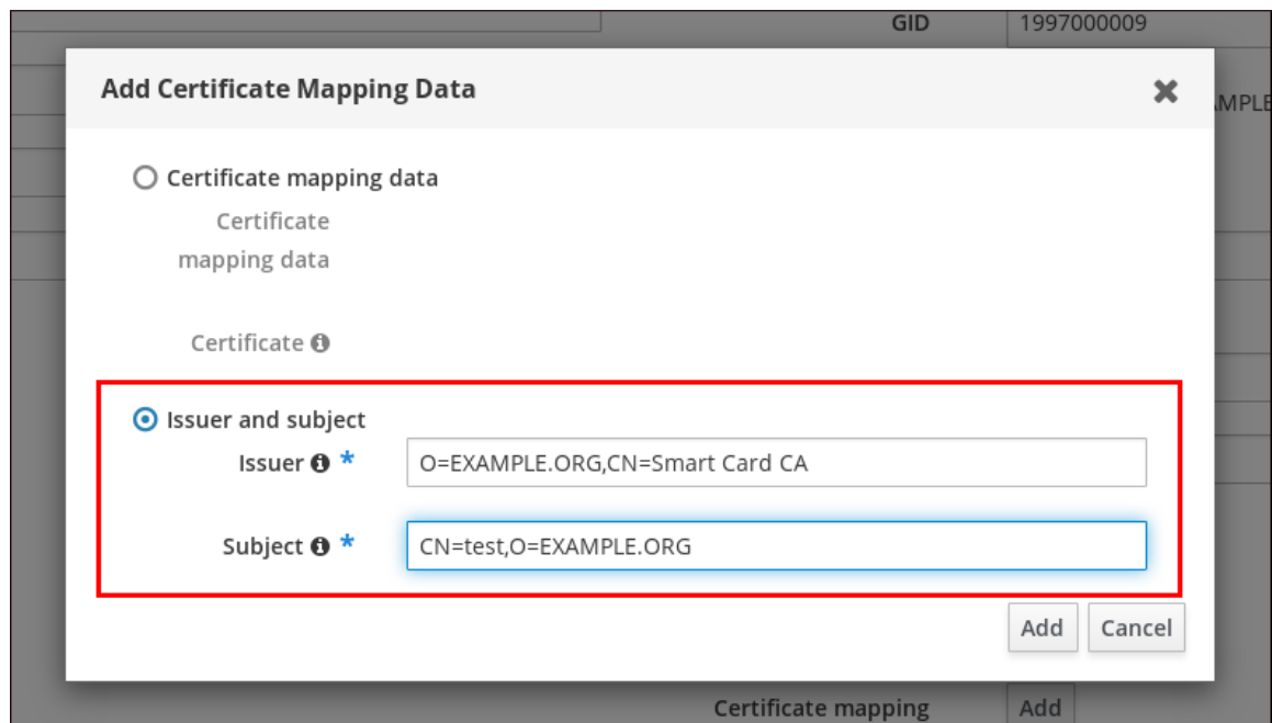
Figure 23.4. Adding a User's Certificate Mapping Data: Issuer and Subject
