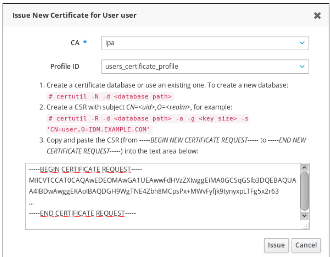
Figure 24.18. Issuing a Certificate for a User
