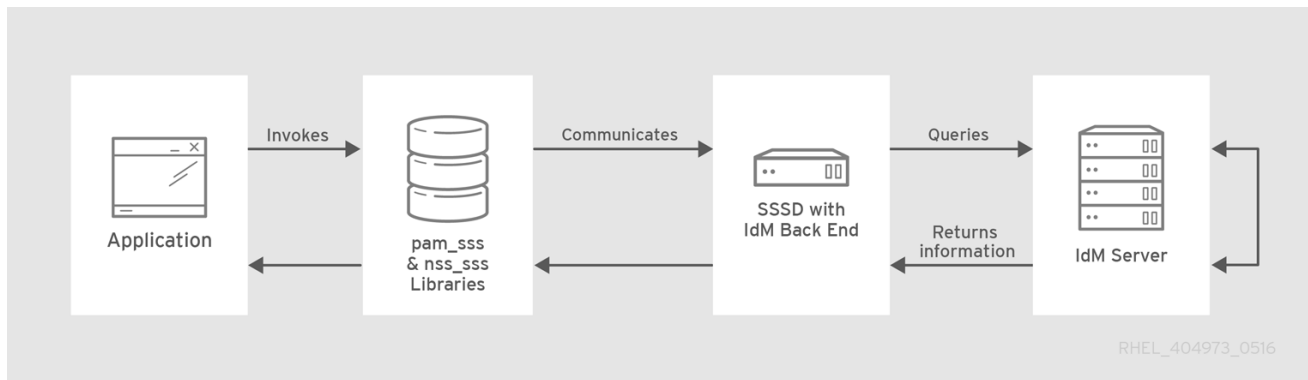
Figure 39.2. Clients and SSSD with an IdM Back End
