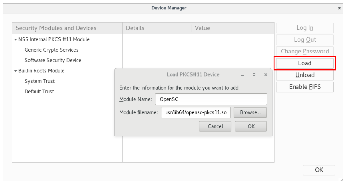
Figure 23.17. Device Manager in Firefox
