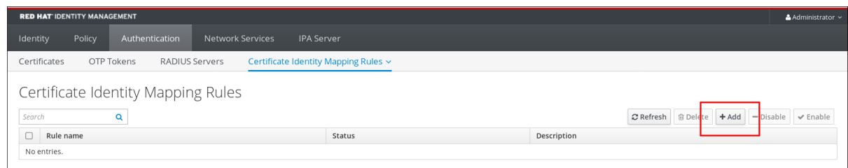
Figure 23.9. Adding a New Certificate Mapping Rule in the IdM Web UI
