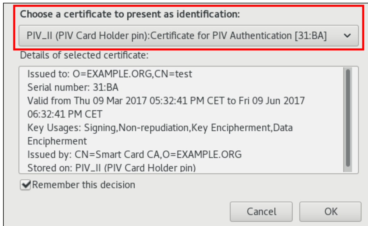
Figure 23.20. Selecting the smart card certificate
