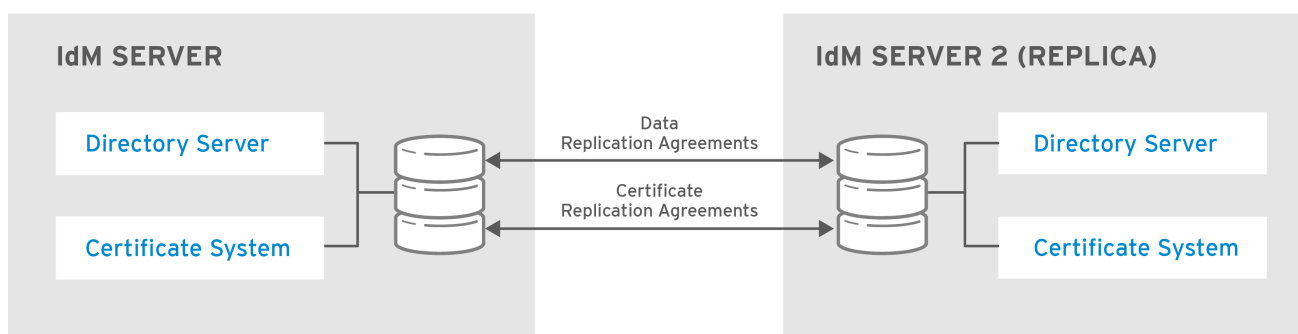
Figure 4.1. Server and Replica Agreements
