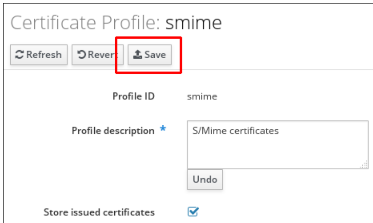
Figure 24.8. Modifying a Certificate Profile in the Web UI
