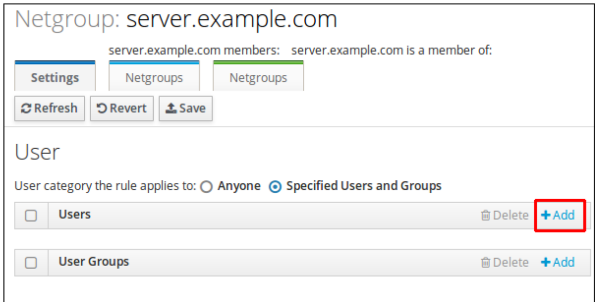
Figure 21.2. User Menu in the Netgroup Tab
