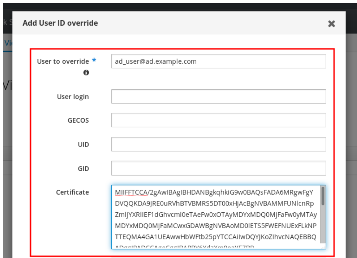
Figure 23.12. Configuring the User ID Override for an AD User
