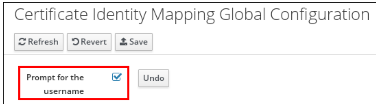
Figure 23.15. Enabling user name hints in the web UI
