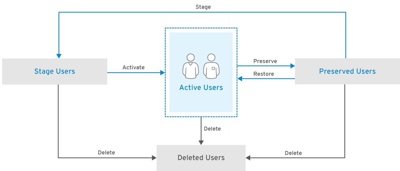
Figure 11.1. User Life Cycle Operations
