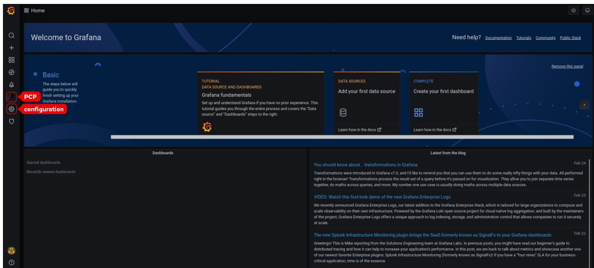
Figure 10.1. Home Dashboard
