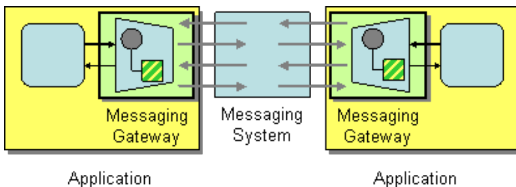
Figure 11.8. Messaging Gateway Pattern
