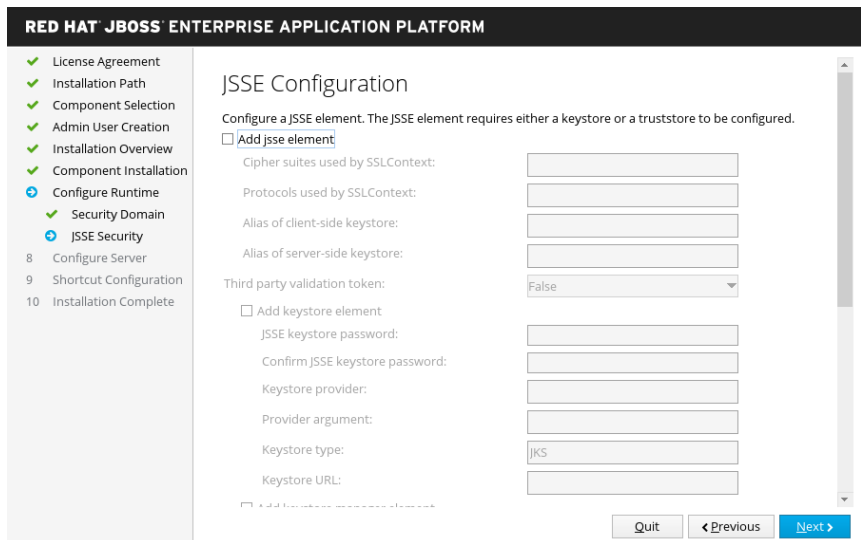
Figure 3.8. JBoss EAP Installer - JSSE Configuration Screen
