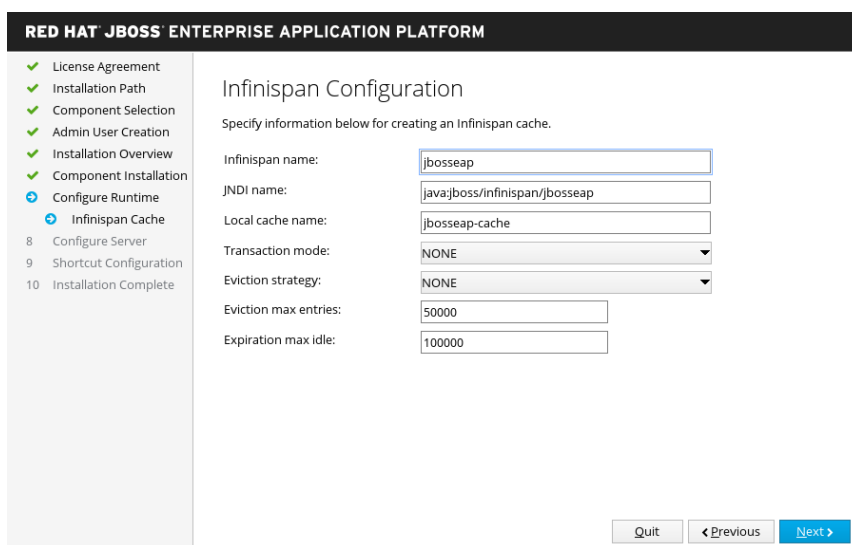
Figure 3.6. JBoss EAP Installer - Infinispan Configuration Screen
