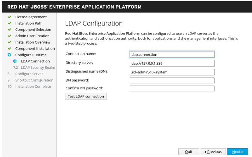
Figure 3.4. JBoss EAP Installer - LDAP Configuration Screen
