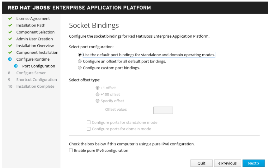
Figure 3.10. JBoss EAP Installer - Socket Bindings Screen
