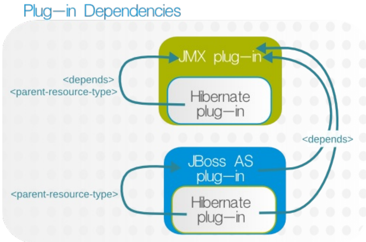
Figure 4.4. Hibernate, JMX, and JBoss AS Dependencies
