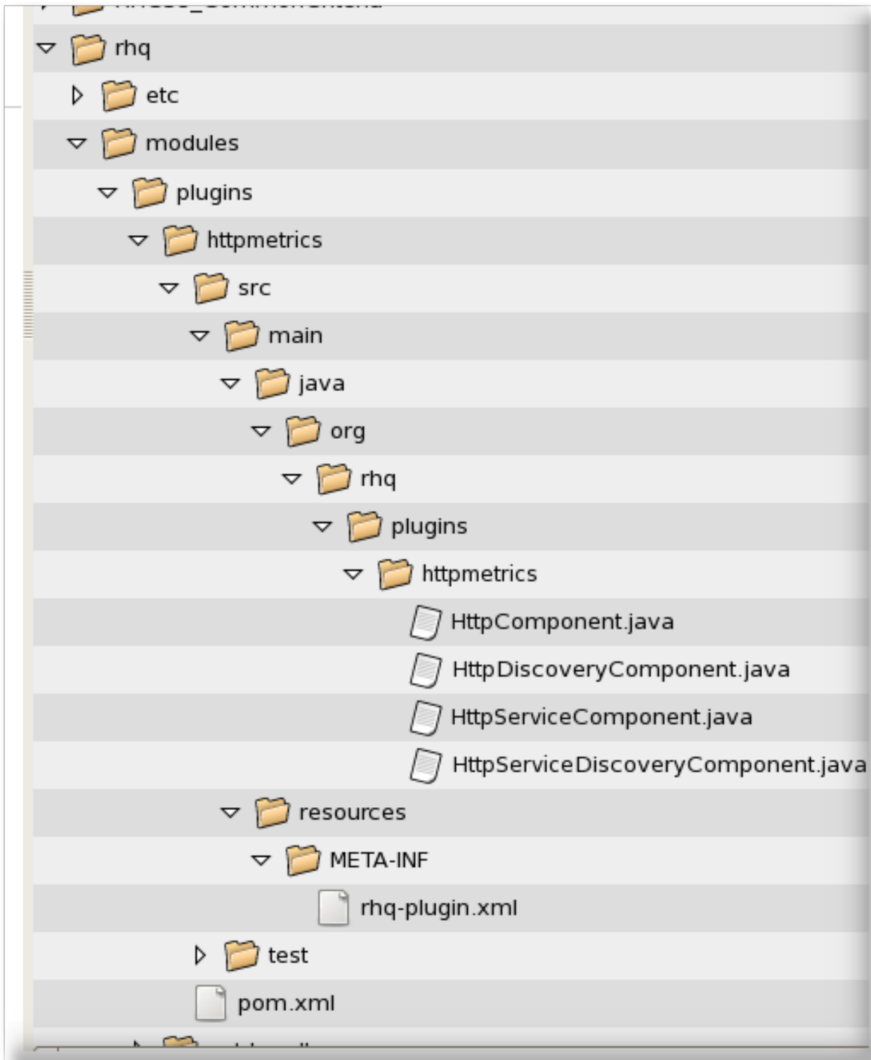
Figure 4.3. Directory Layout of an Agent Plug-in Project
