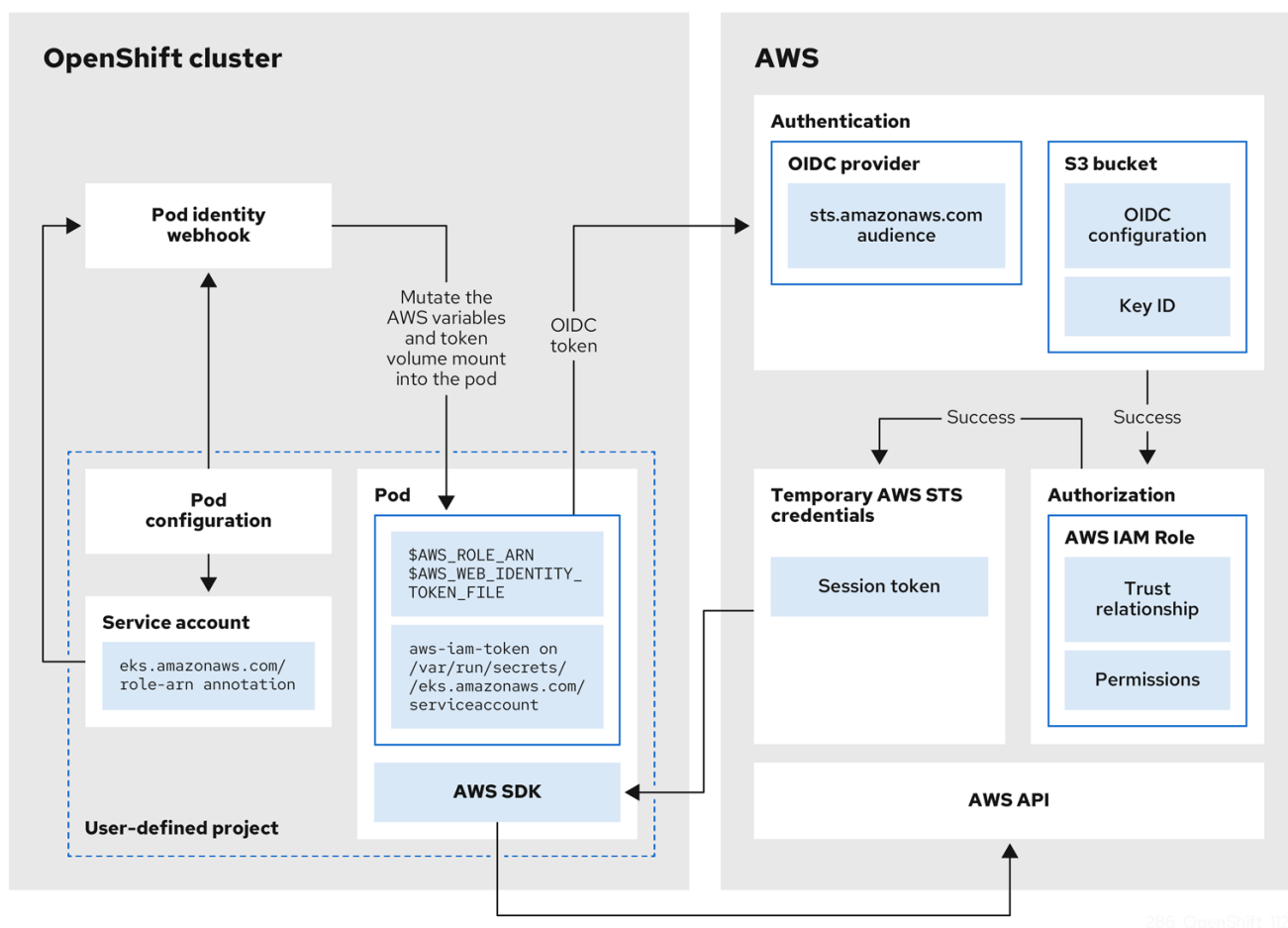
Figure 9.2. Pod identity webhook workflow in user-defined projects
