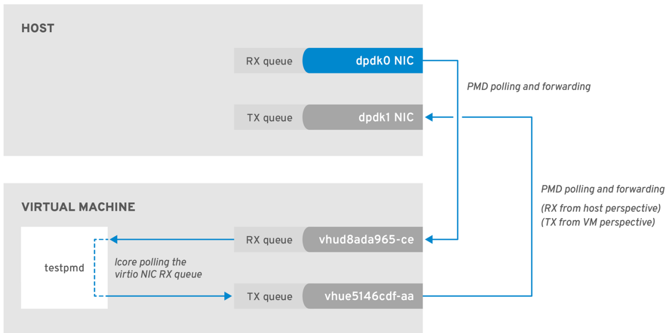
Figure 2.1. Polling the physical adapter RX queue
