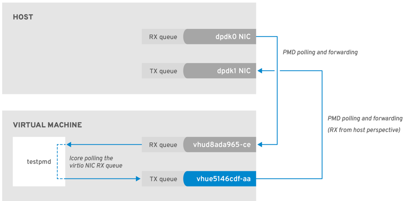
Figure 2.3. Polling the virtual adapter TX queue
