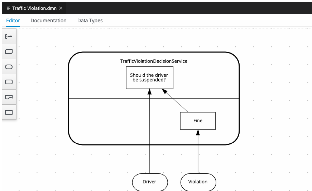
Figure 21.1. Example TrafficViolationDecisionService decision service with single-output decision
