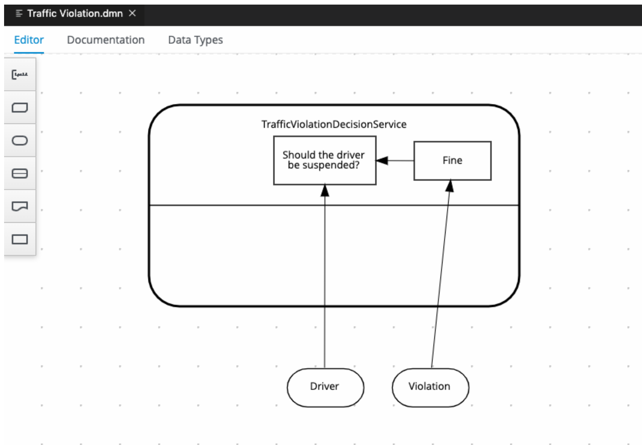
Figure 21.2. Example TrafficViolationDecisionService decision service with multiple-output decision
