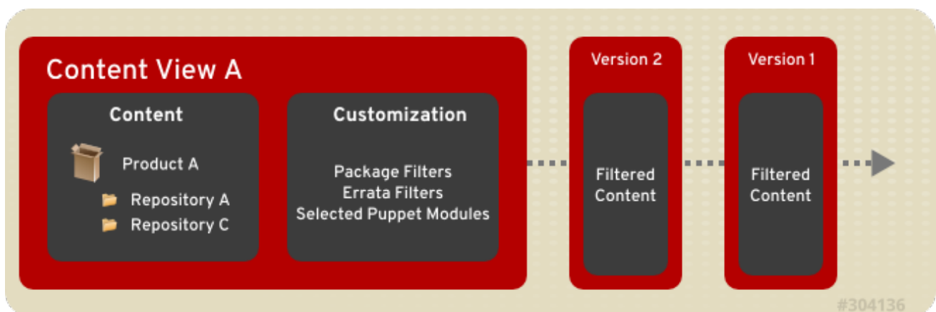
Figure 2.8. Creating New Versions of a Content View
