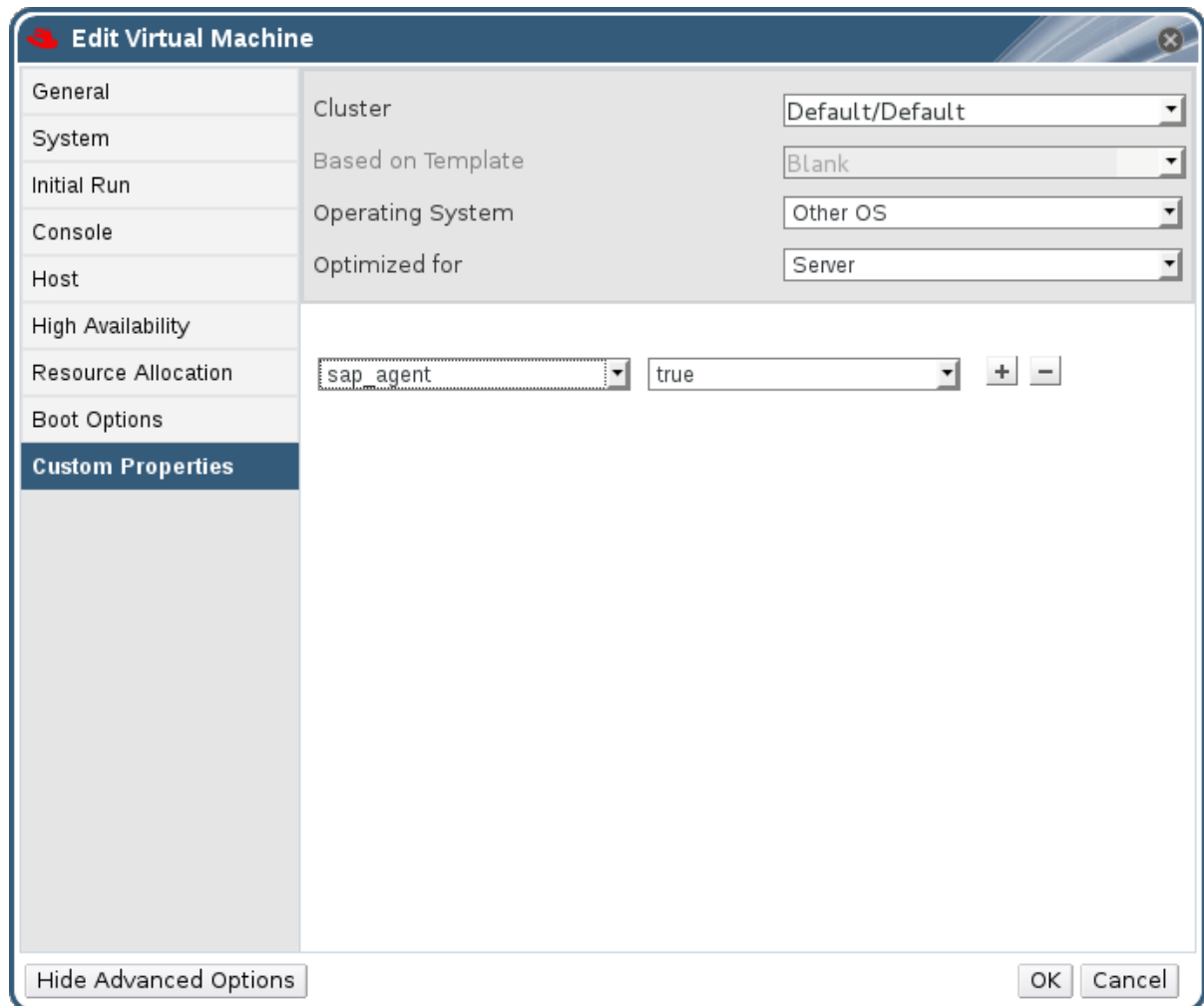
Figure 6.21. Enable SAP
