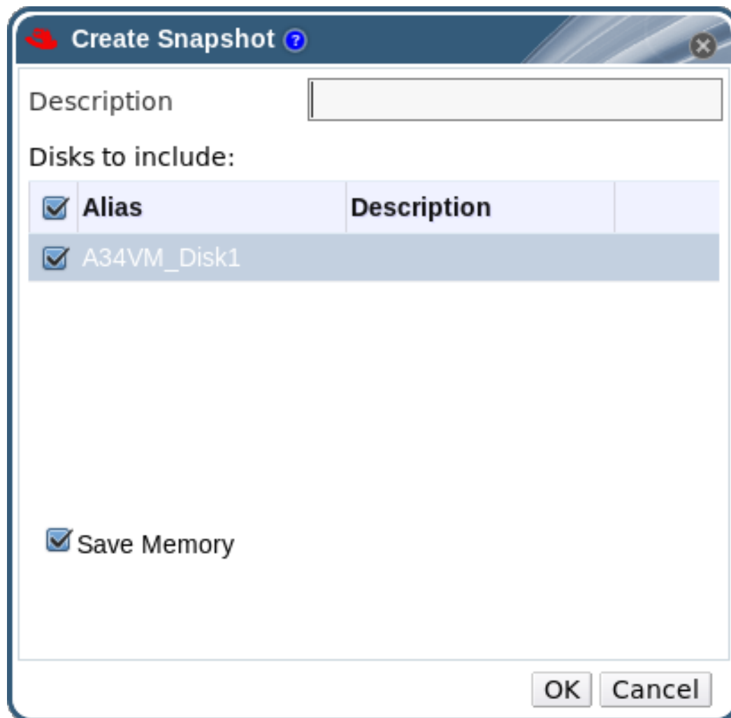
Figure 6.1. Create snapshot
