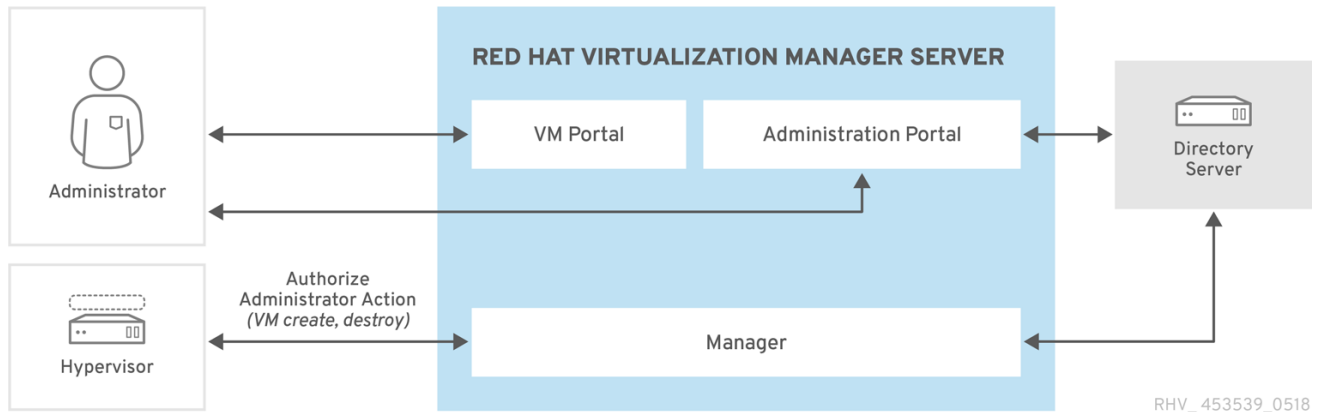
Figure 6.1. GSSAPI Authentication
