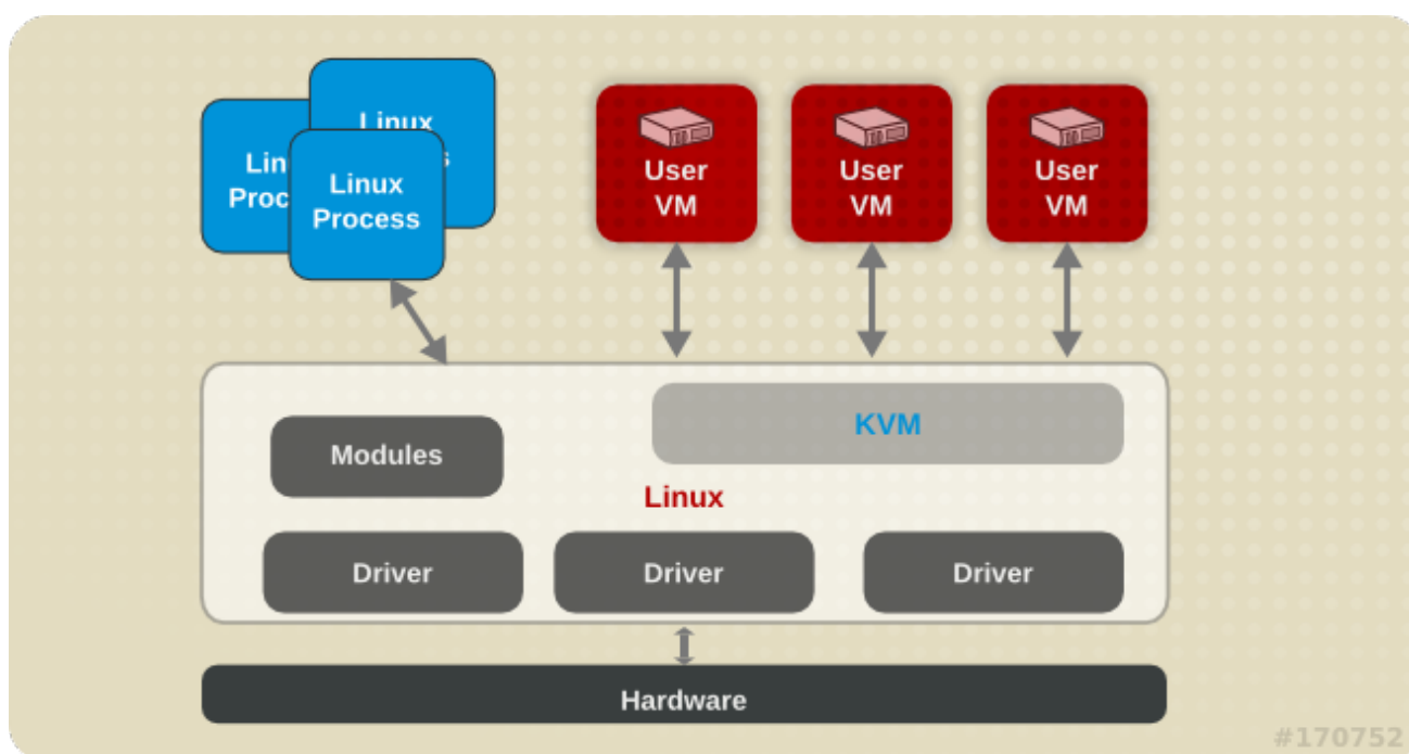
Figure 3.1. KVM architecture
