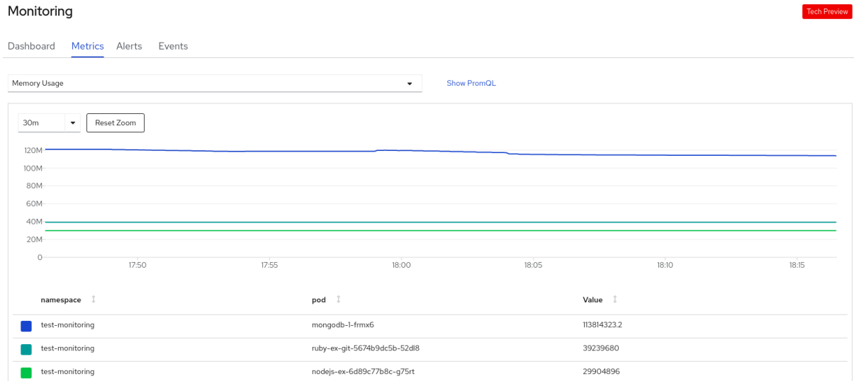
Figure 11.1. Monitoring metrics
