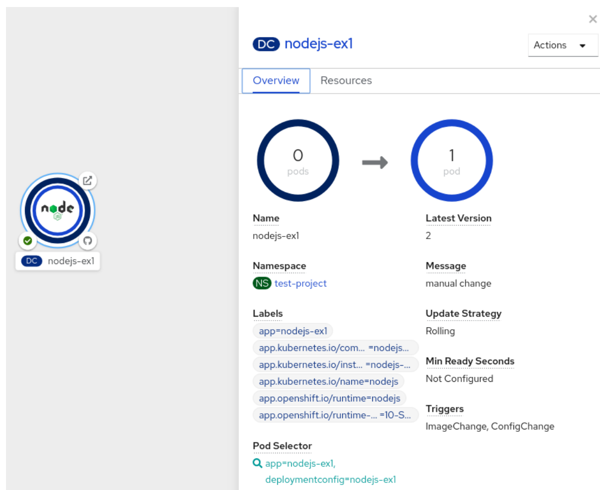
Figure 8.1. Rolling update
