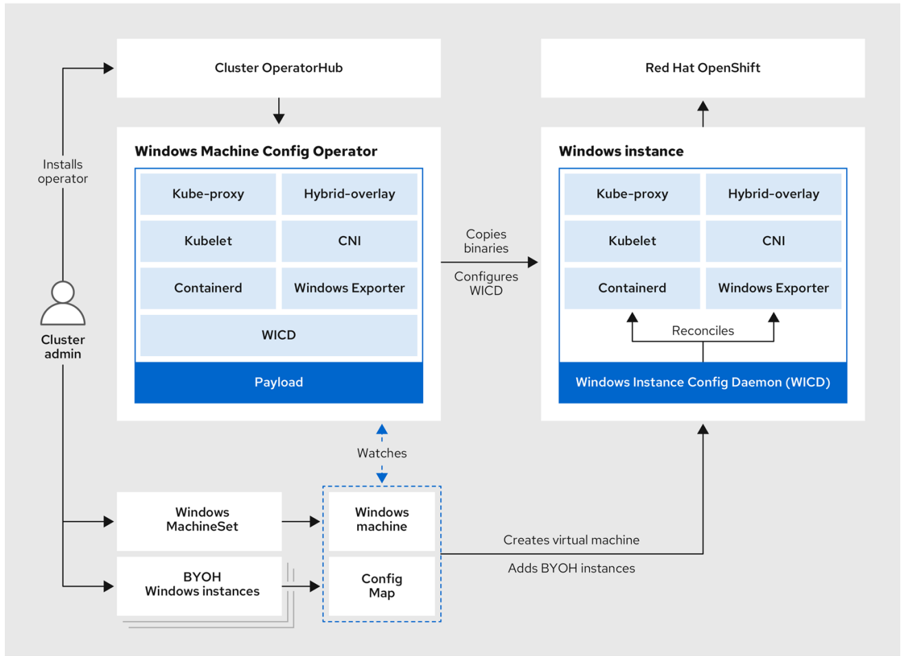
Figure 4.1. WMCO design
