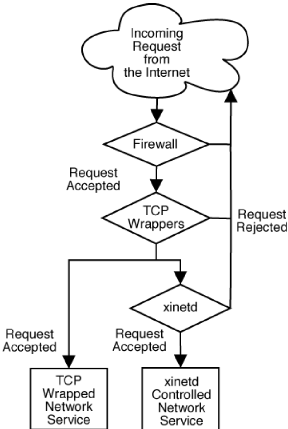
Figure 17.1. Access Control to Network Services
