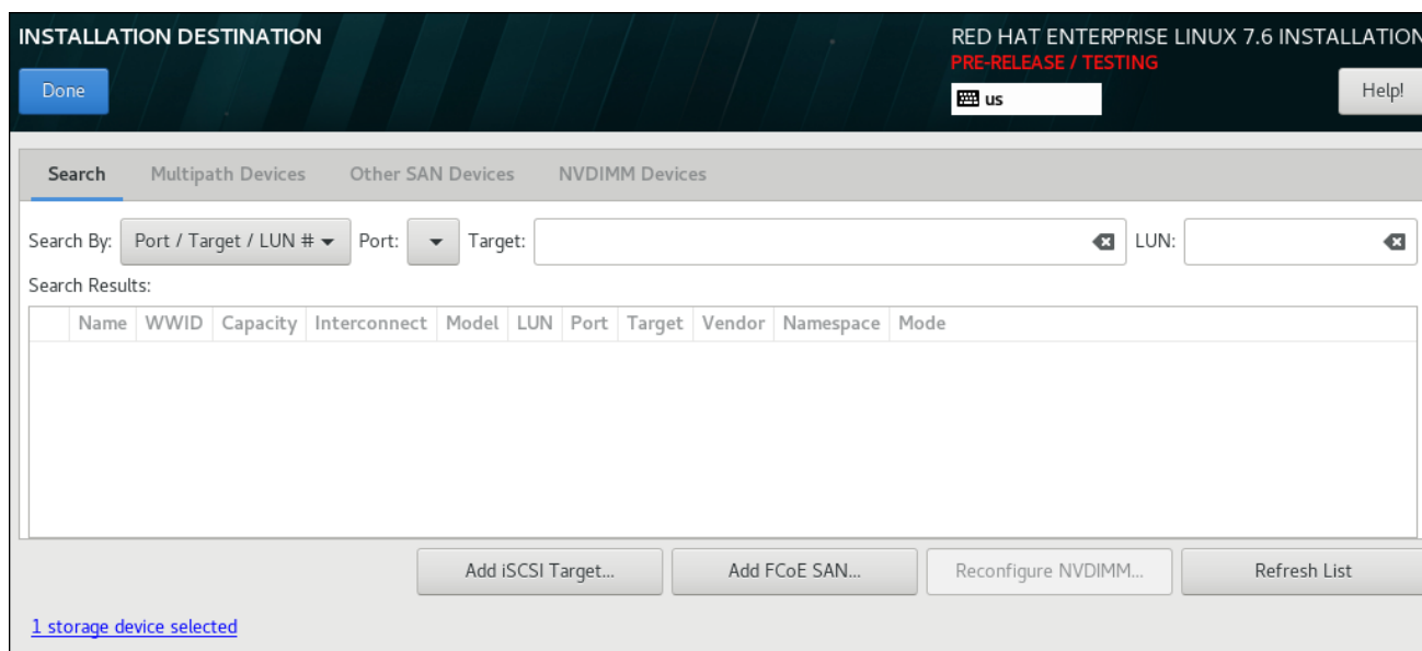
Figure 8.31. Advanced Storage Options
