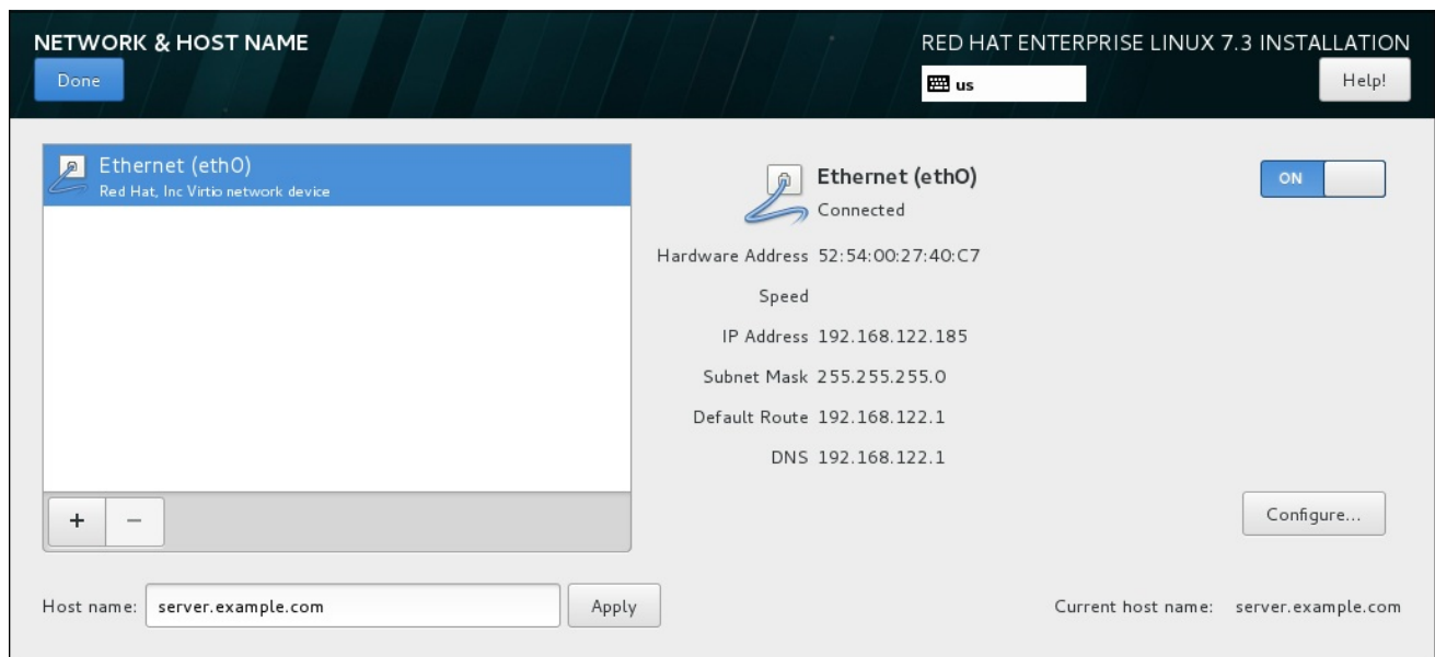
Figure 18.9. Network & Hostname Configuration Screen
