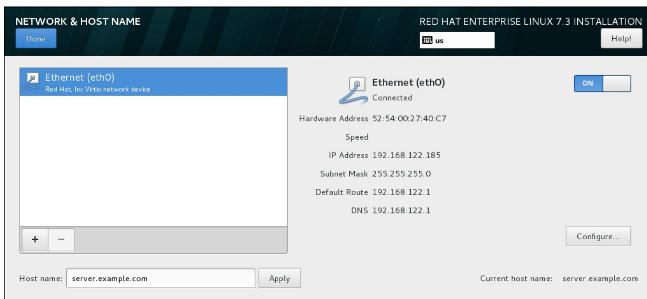
Figure 13.10. Network & Hostname Configuration Screen
