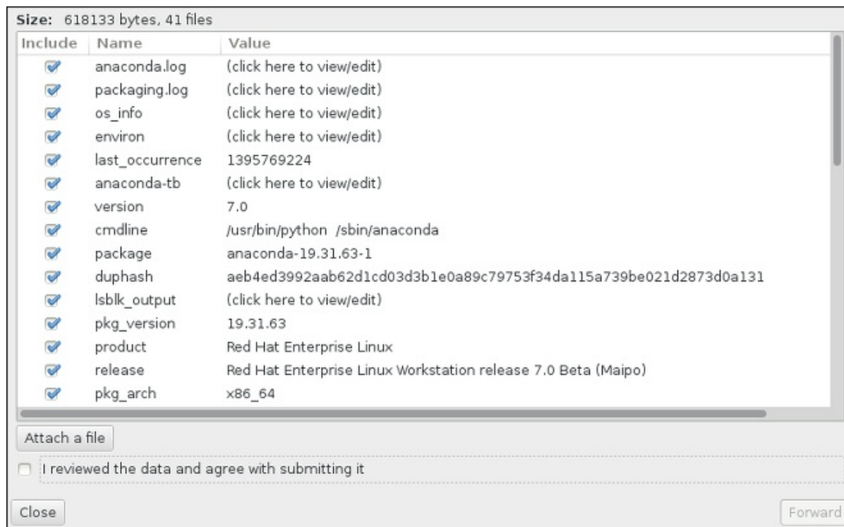
Figure 9.7. Review the Files to Be Sent
