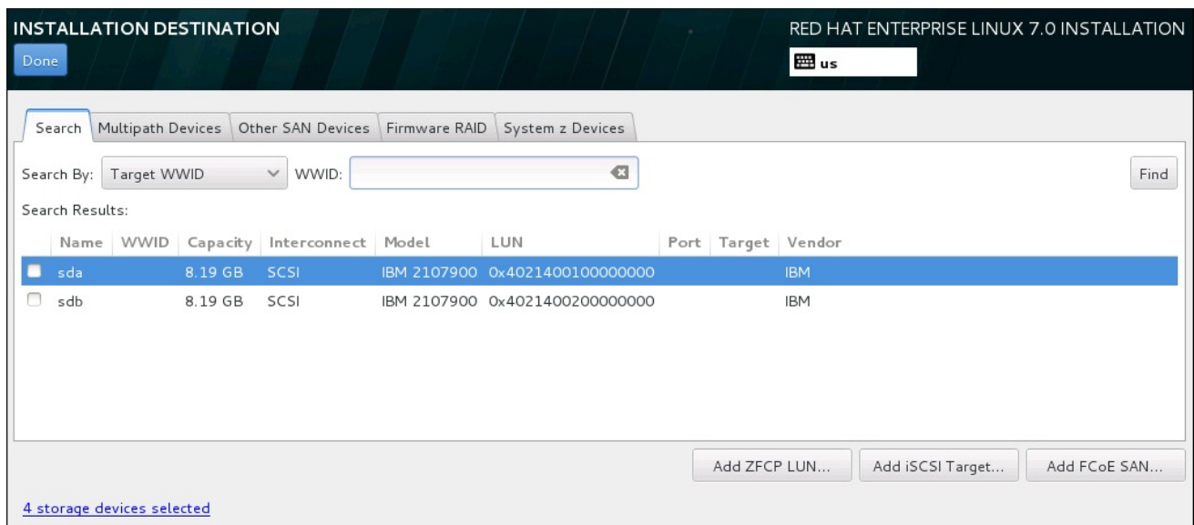
Figure 18.29. Advanced Storage Options
