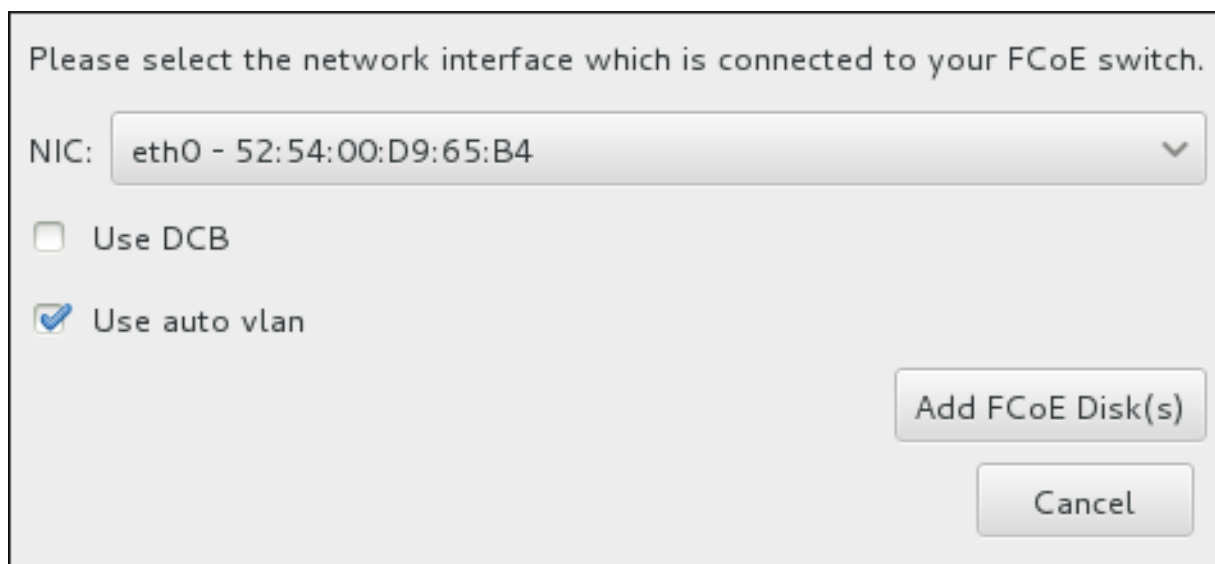
Figure 13.34. Configure FCoE Parameters
