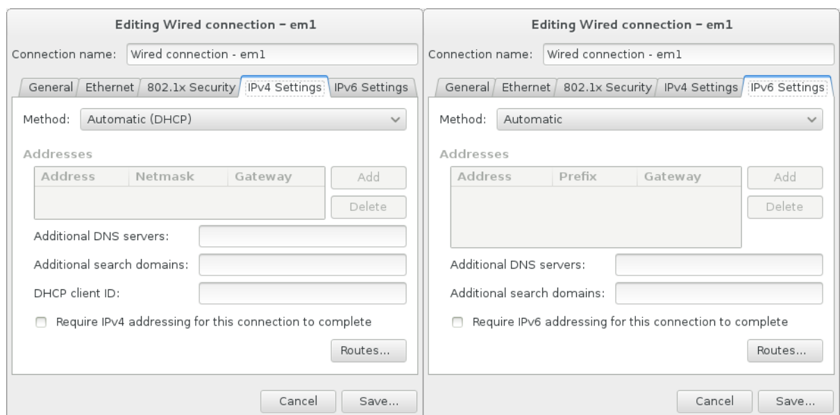
Figure 18.11. IP Protocol Settings
