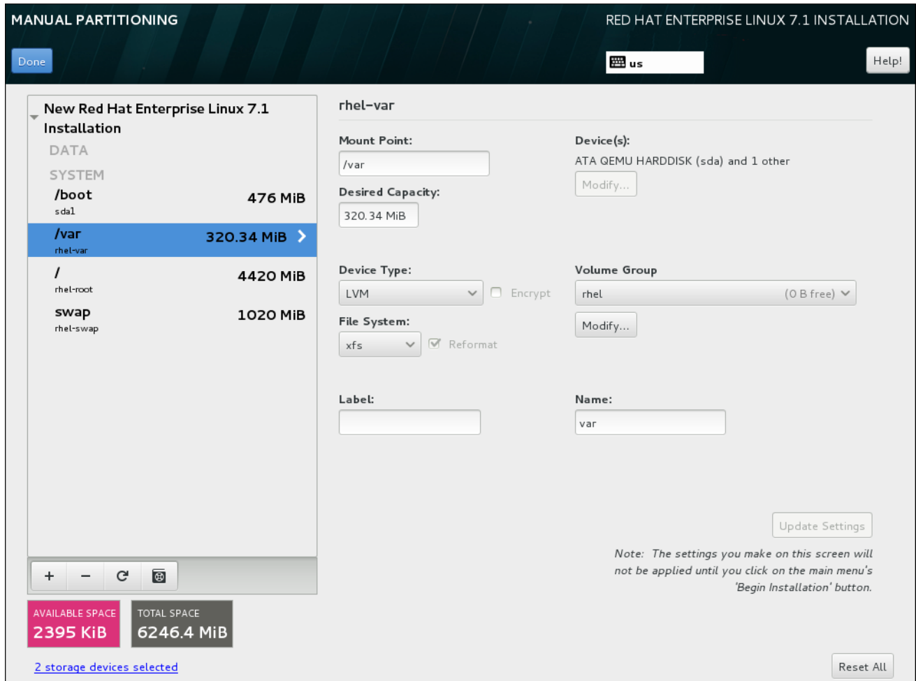
Figure 18.23. Configuring a Logical Volume
