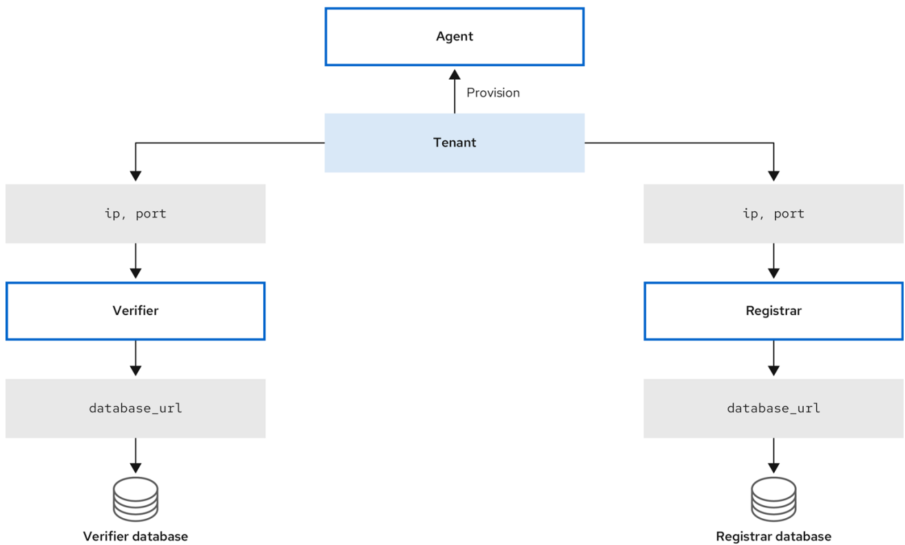
Figure 7.1. Connections between Keylime components through configurations
