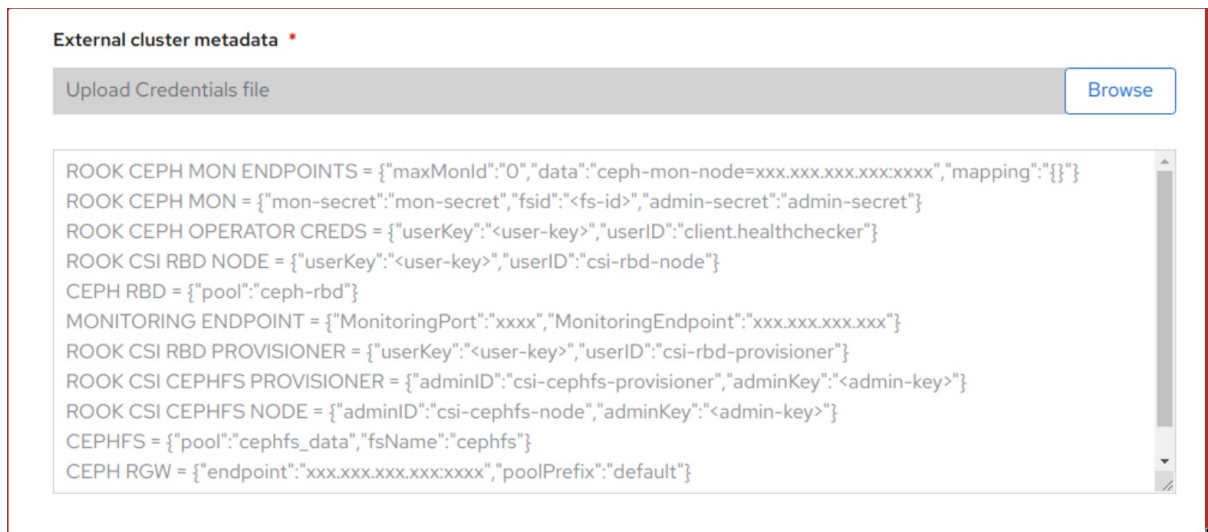
Figure 4.2. Json file content
