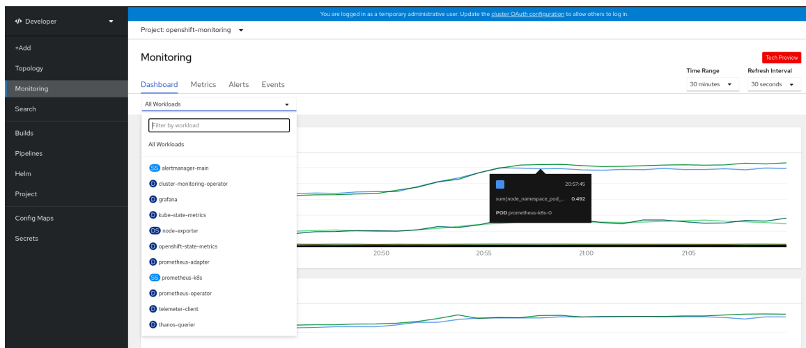
図7.1 Monitoring dashboard
