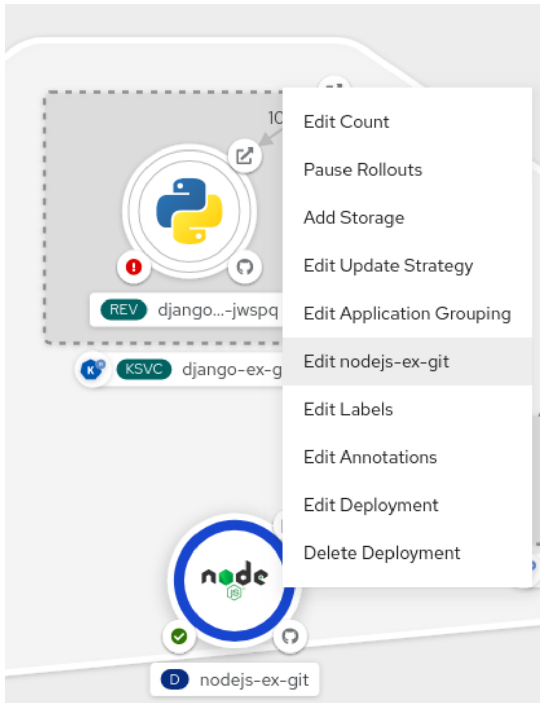
図3.6 Edit application
