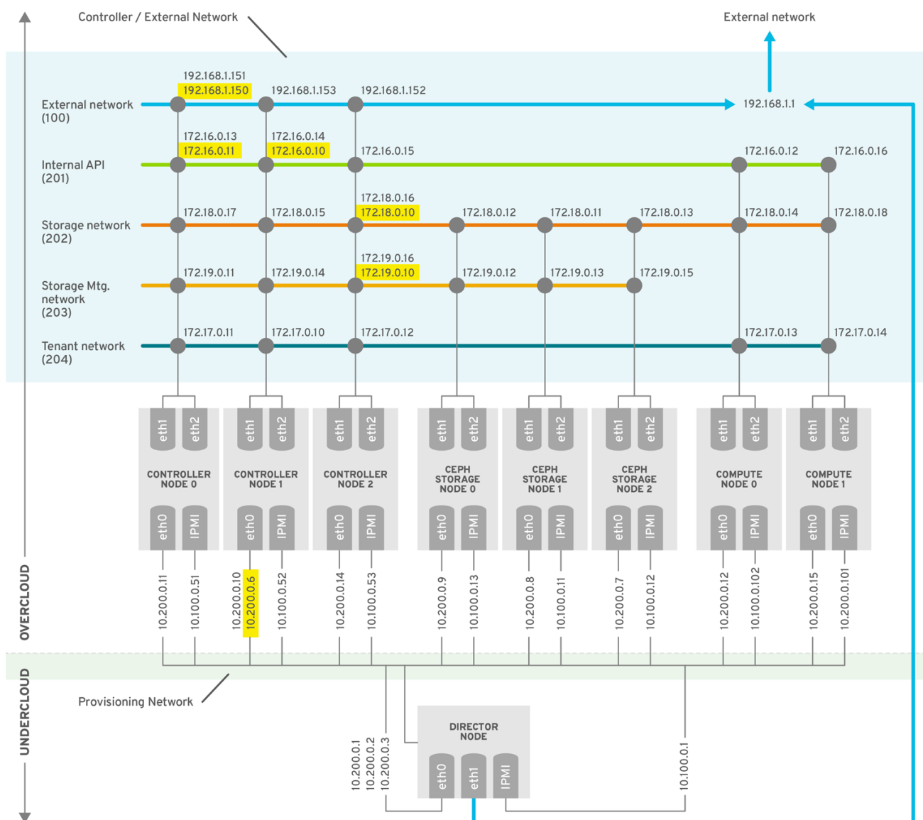
图2.1 Example high availability deployment architecture
