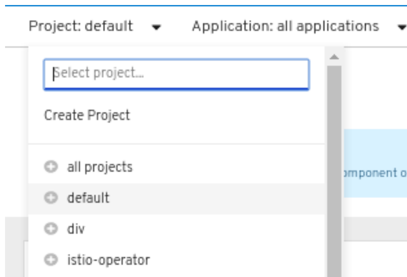
図2.1 Create project
