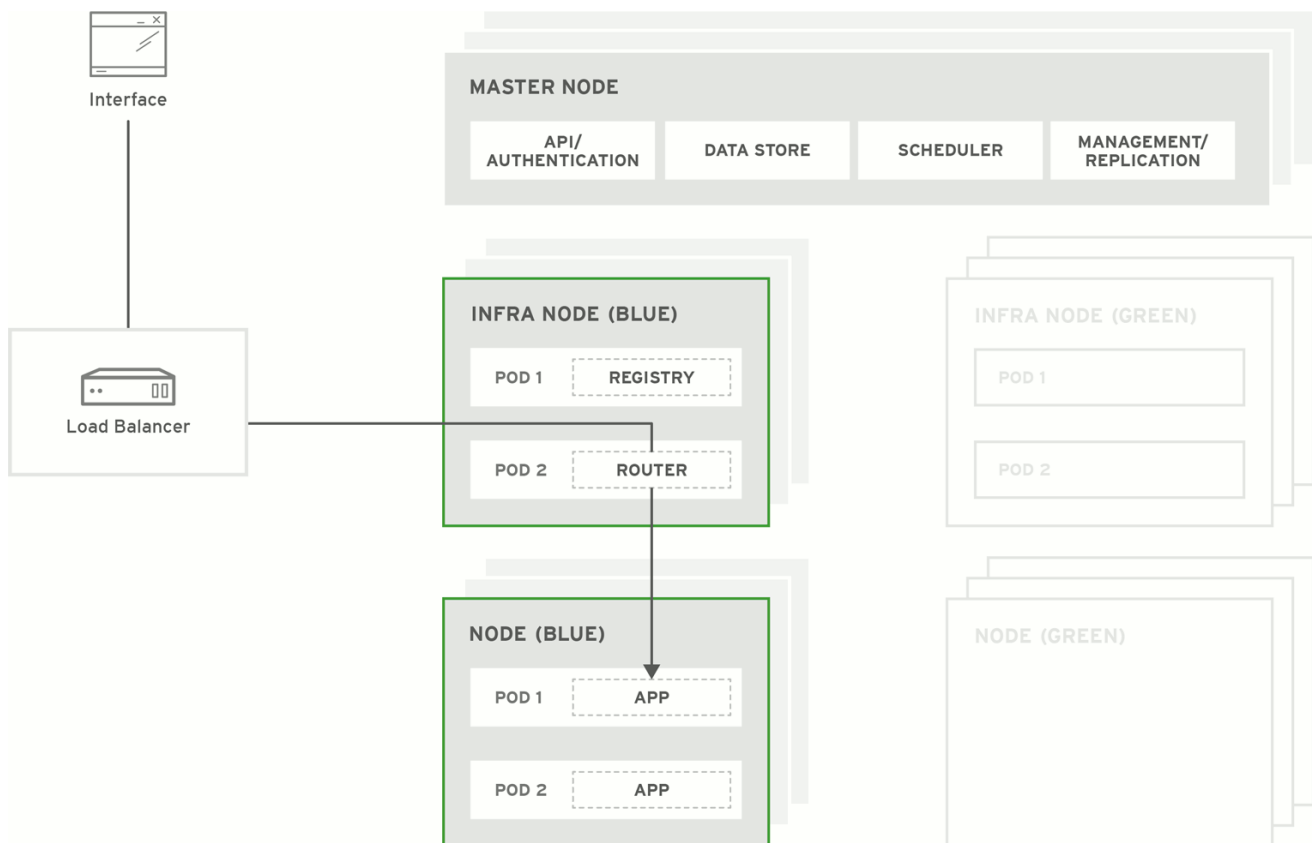
图 3.1. Blue-green deployment
