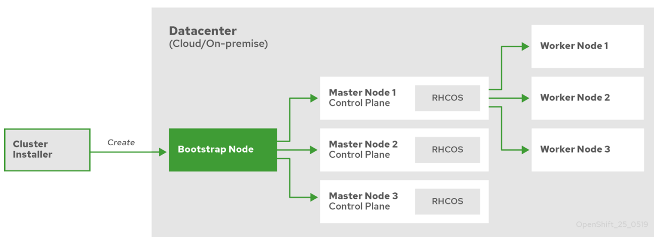
图 2.2. Creating the bootstrap, master, and worker machines
