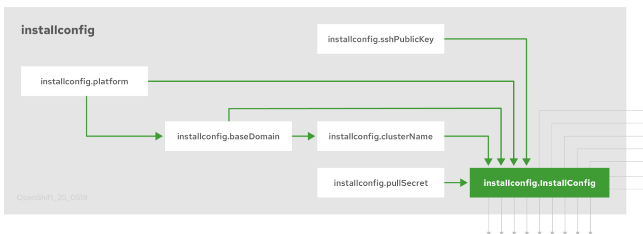
图 2.1. OpenShift Container Platform installation targets and dependencies
