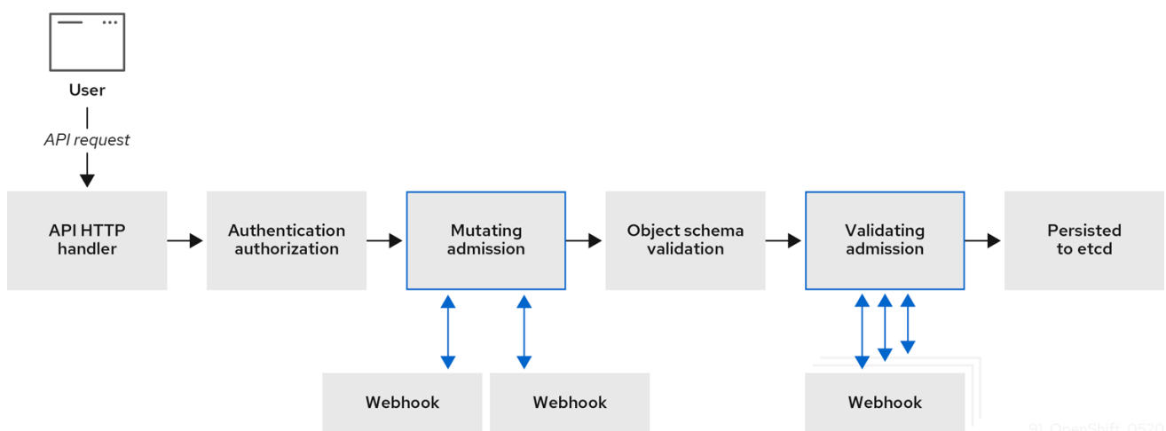
图 8.1. API admission chain with mutating and validating admission plug-ins
