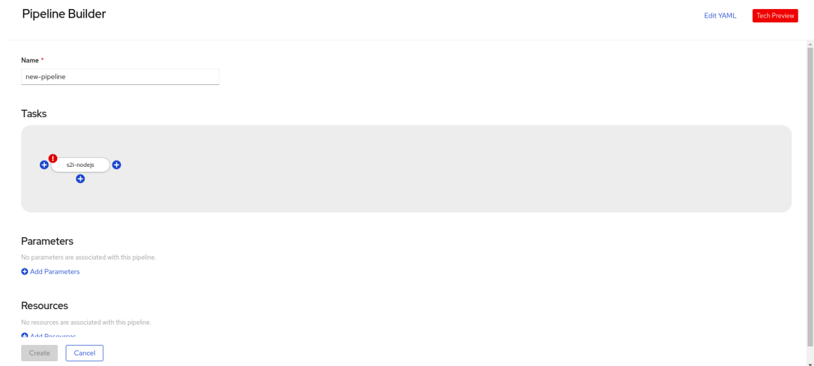
图 5.1. Pipeline Builder
