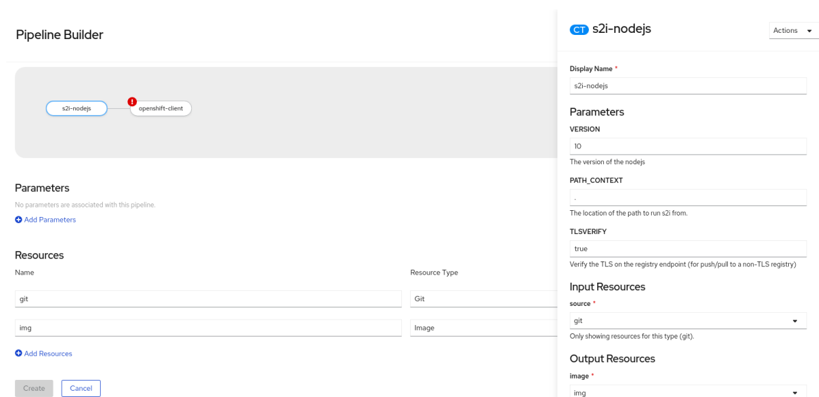
图 5.2. Tasks details in Pipelines Builder
