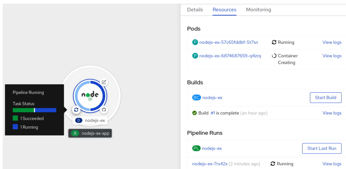
图 5.5. Pipelines on the Topology view
