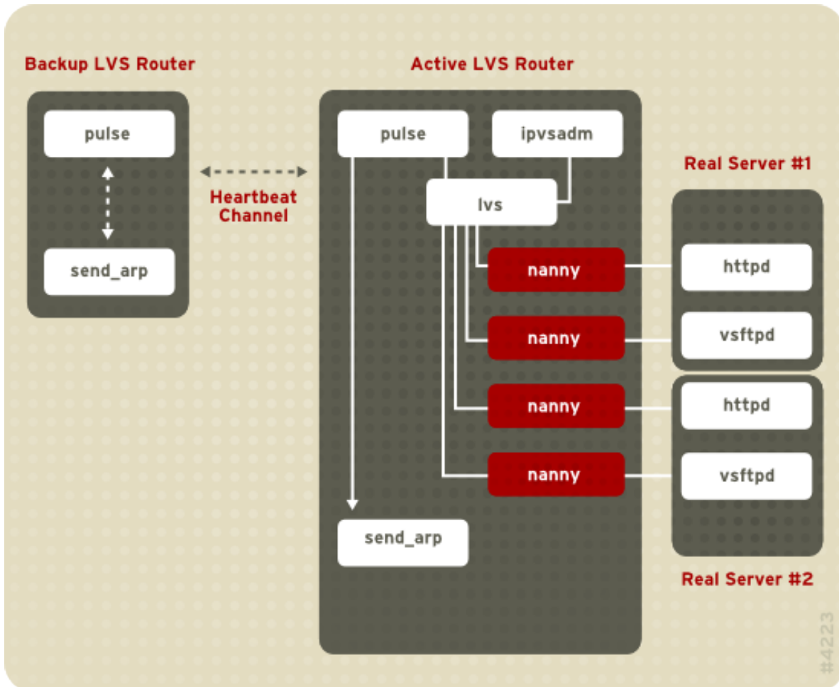
Figure 1.5. LVS Components
