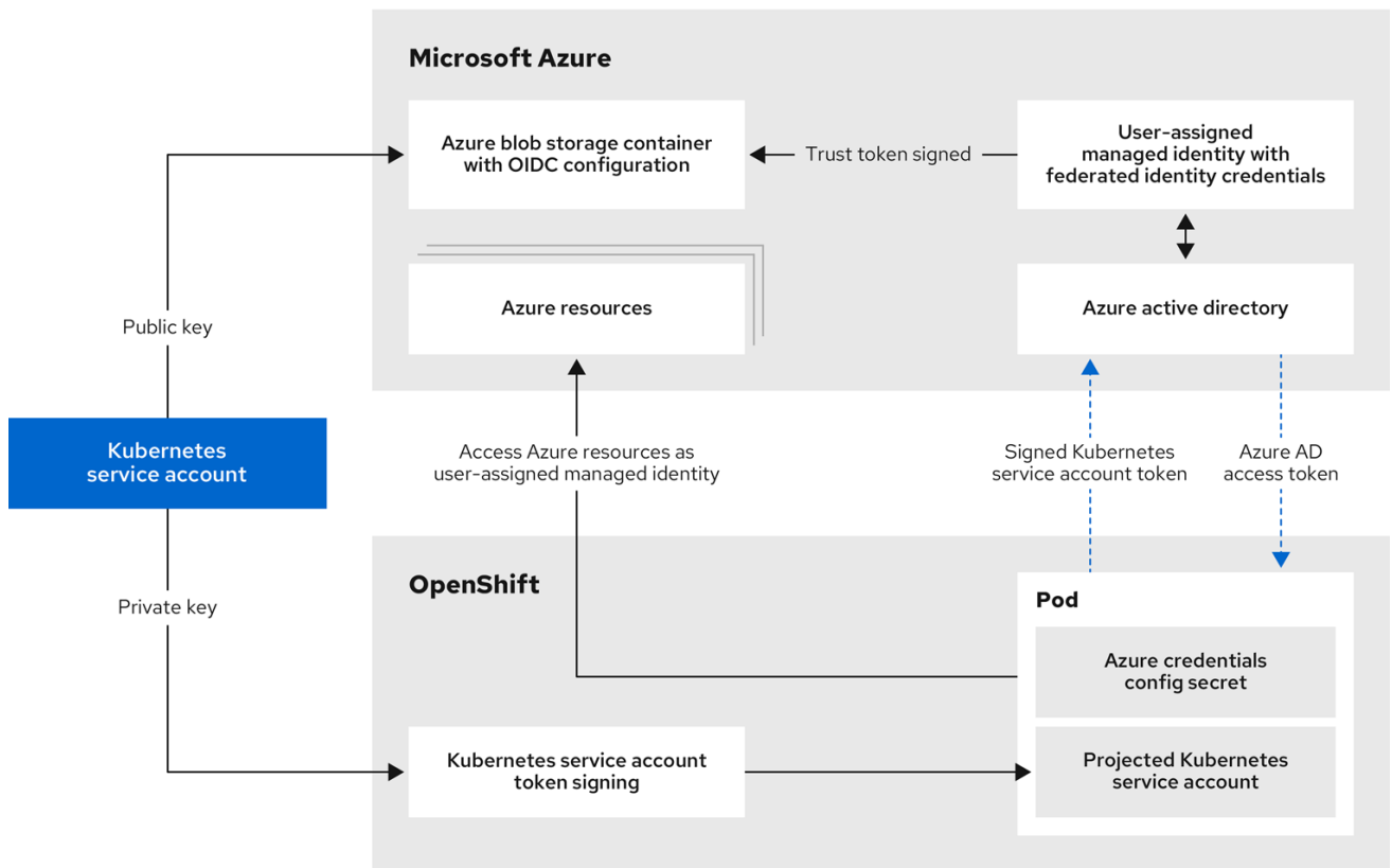
Figure 20.4. Workload ID authentication flow
