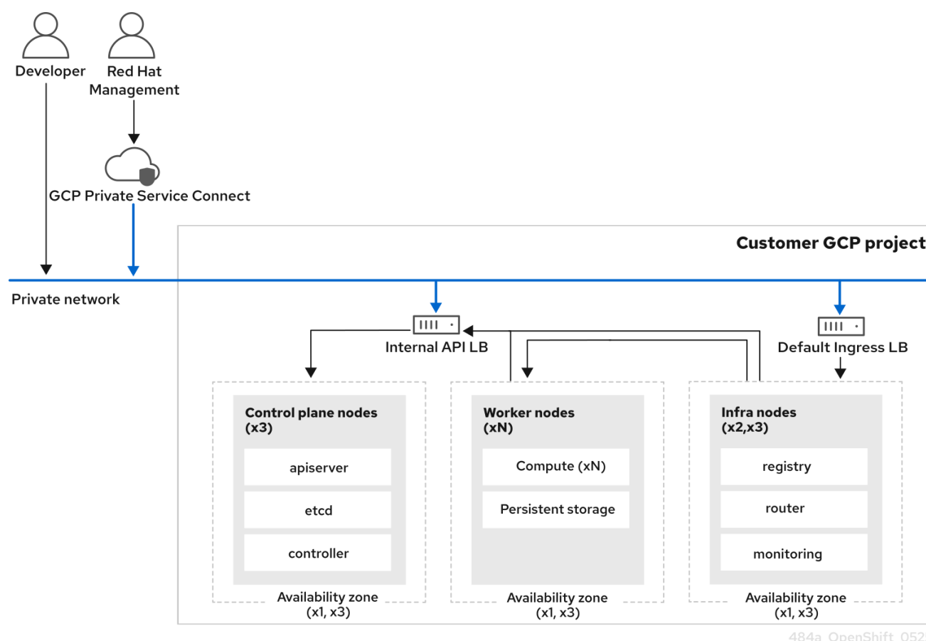
Figure 3.2. OpenShift Dedicated on Google Cloud Platform (GCP) deployed on a private network with PSC
