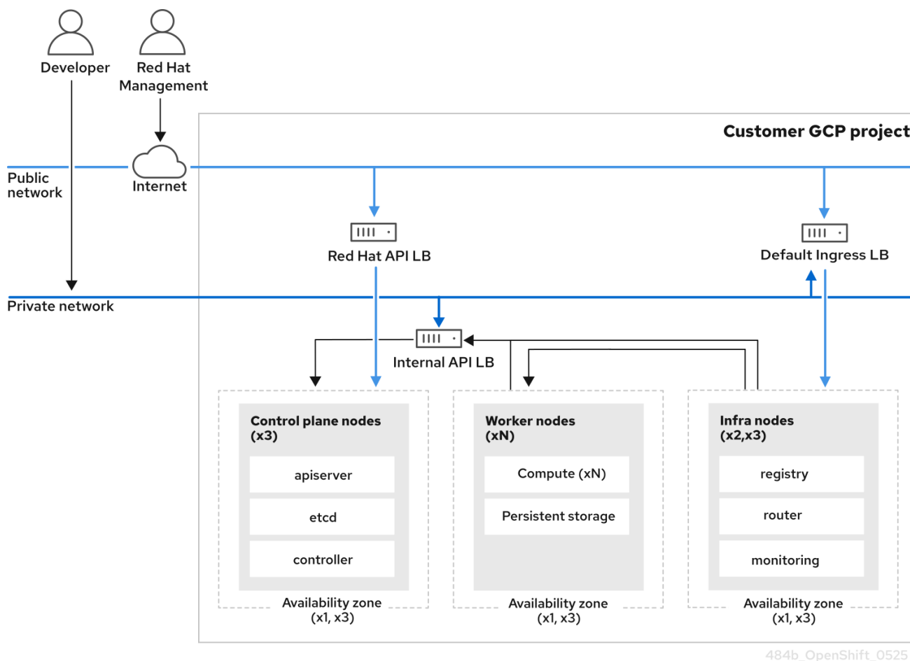
Figure 3.3. OpenShift Dedicated on Google Cloud Platform (GCP) deployed on a private network without PSC
