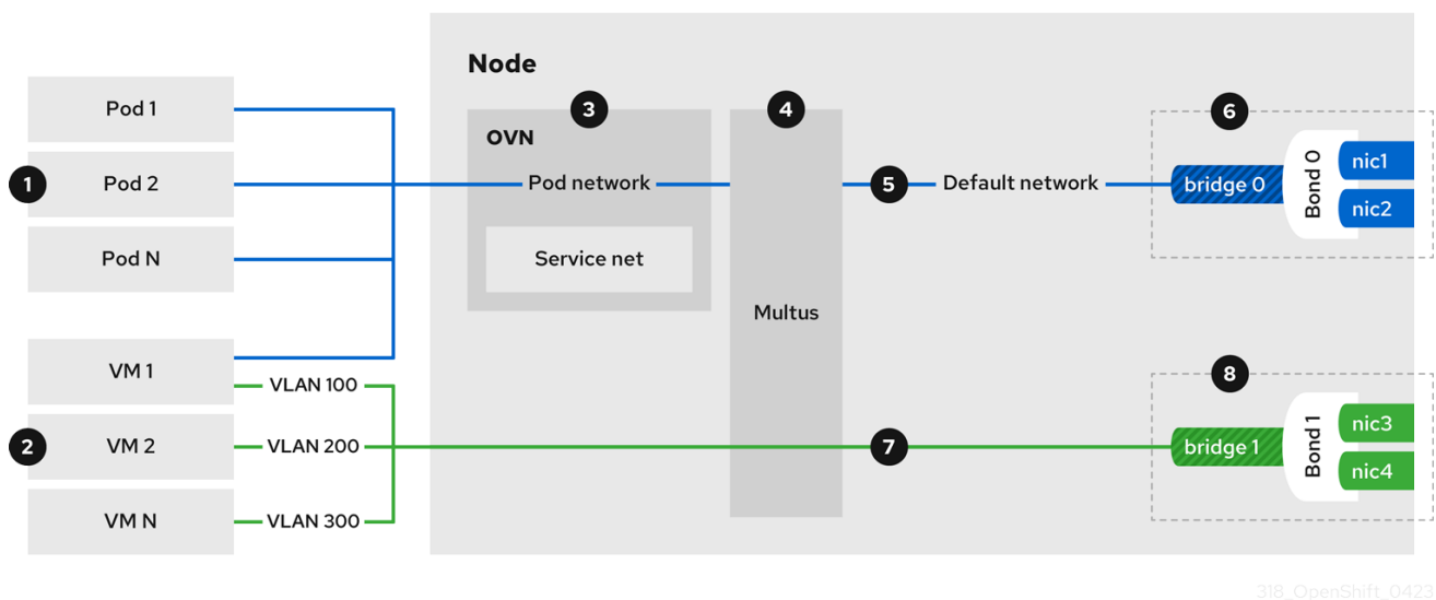
Figure 10.1. OpenShift Virtualization networking overview
